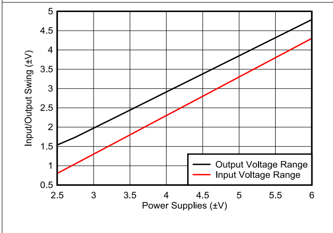
5-27. Common-Mode Input and Output Swing vs Supply Voltage
