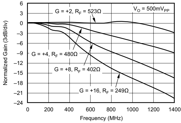
5-39. Noninverting Small-Signal Frequency Response
