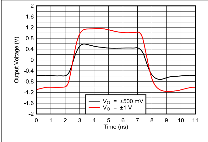
5-31. Noninverting Pulse Response
