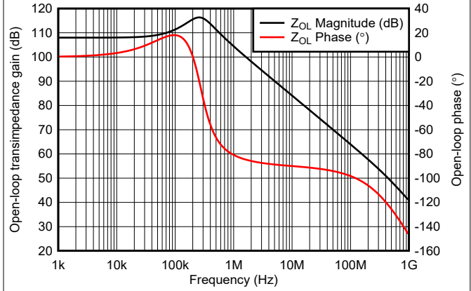
图 5-20. Open-Loop Transimpedance Gain and Phase
