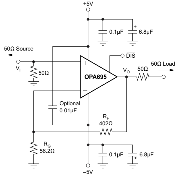
図 6-1. DC-Coupled, G = +8 V/V, Bipolar Supply Specifications and Test Circuit
