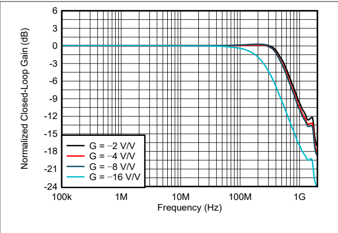
5-30. Inverting Small-Signal Frequency Response
