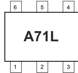
図 4-2. DBV Package, 6-Pin SOT-23 (Top View)
