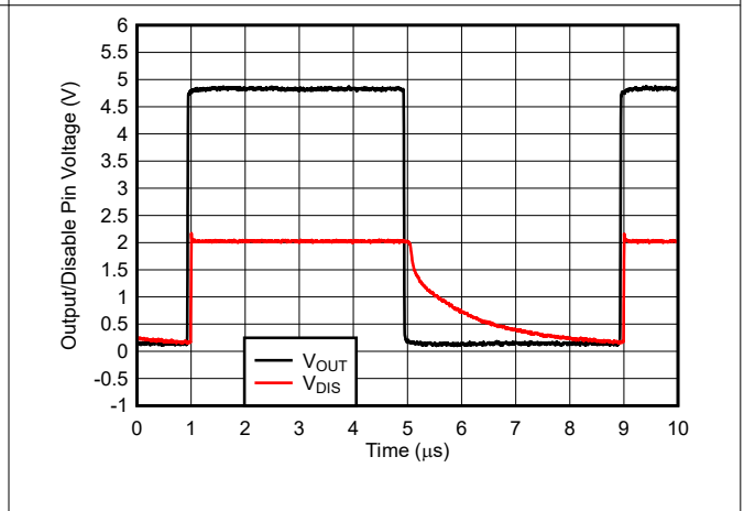
5-28. Large-Signal Disable and Enable Response
