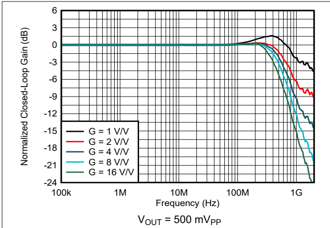
5-29. Noninverting Small-Signal Frequency Response
