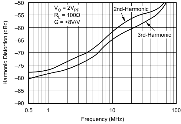
5-75. Harmonic Distortion vs Frequency
