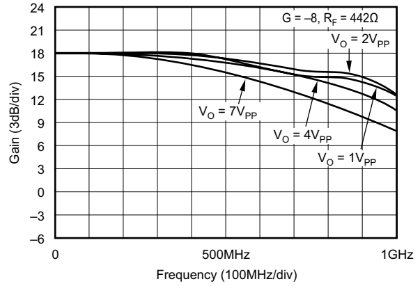
5-40. Inverting Small-Signal Frequency Response
