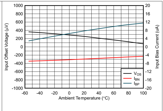
5-26. Typical DC Drift Over Temperature
