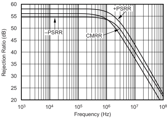
Figure 5-57. CMRR and PSRR vs Frequency
