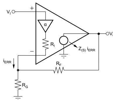
図 7-1. Current-Feedback Transfer Function Analysis Circuit
