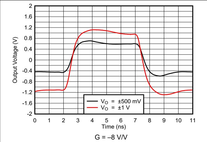
5-32. Inverting Pulse Response
