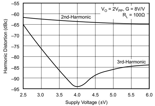
5-46. 10-MHz Harmonic Distortion vs Supply Voltage
