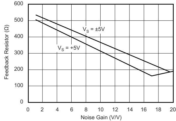
図 7-2. Recommended Feedback Resistor vs Noise Gain
