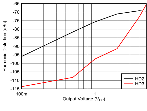
Figure 5-10. 10-MHz Harmonic Distortion vs Output Voltage
