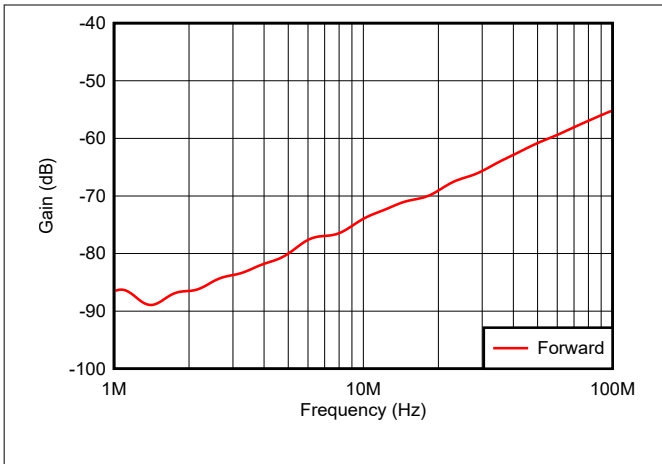
5-25. Disabled Feedthrough vs Frequency
