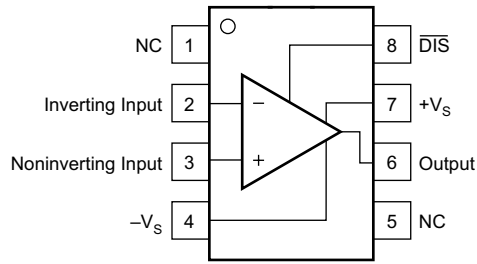
図 4-1. D Package, 8-Pin SOIC, and DGK Package, 8-Pin VSSOP (Top View)
