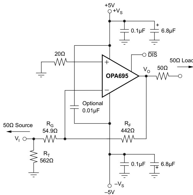
図 6-2. DC-Coupled, G = -8 V/V, Bipolar Supply Specifications and Test Circuit
