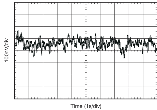
6-8. 0.1-Hz to 10-Hz Noise
