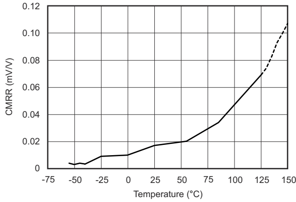
6-7. Common-Mode Rejection Ratio vs Temperature
