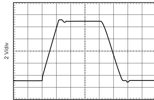
Time (400 ns/div)
