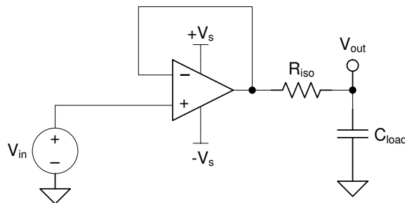
7-7. Extending Capacitive Load Drive With the OPA4991-EP
