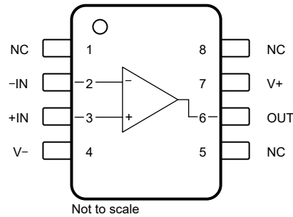
FIG 5-1. OPA197-Q1 DGK Package, 8-Pin VSSOP, Top View
