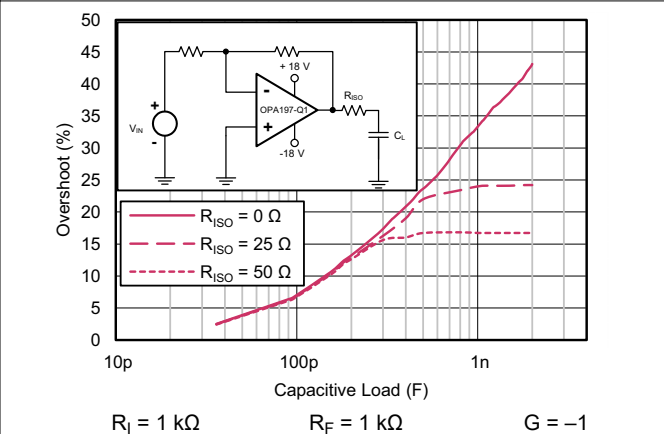
6-30. Small-Signal Overshoot vs Capacitive Load (100-mV Output Step)
