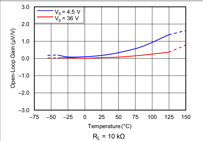
6-28. Open-Loop Gain vs Temperature
