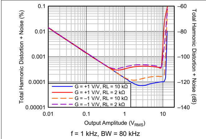
6-25. THD+N vs Output Amplitude
