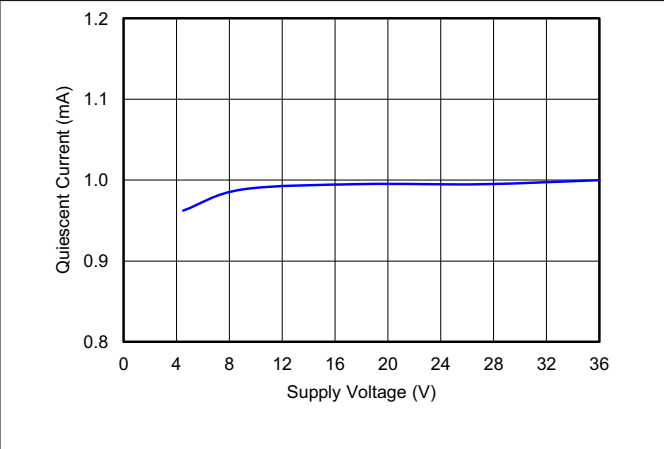
6-26. Quiescent Current vs Supply Voltage
