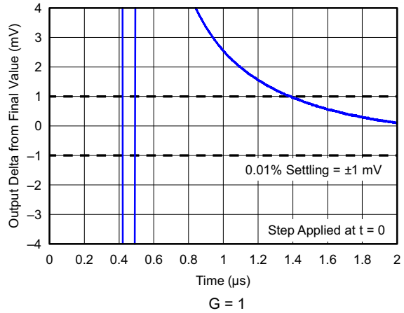
6-40. Settling Time (10-V Negative Step)
