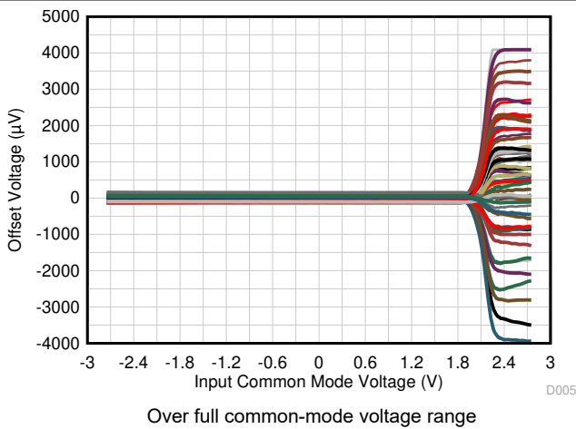
7-43. Offset Voltage vs Common-Mode Voltage (Full Range)
