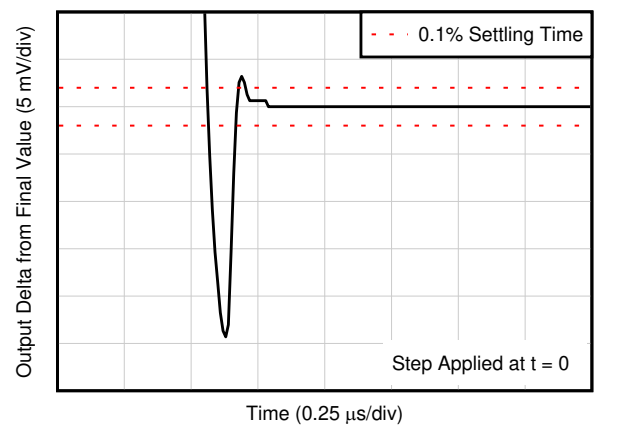
C_L = 20\text{ pF} , Gain = 1, V_{IN} = 2\text{-V step}
