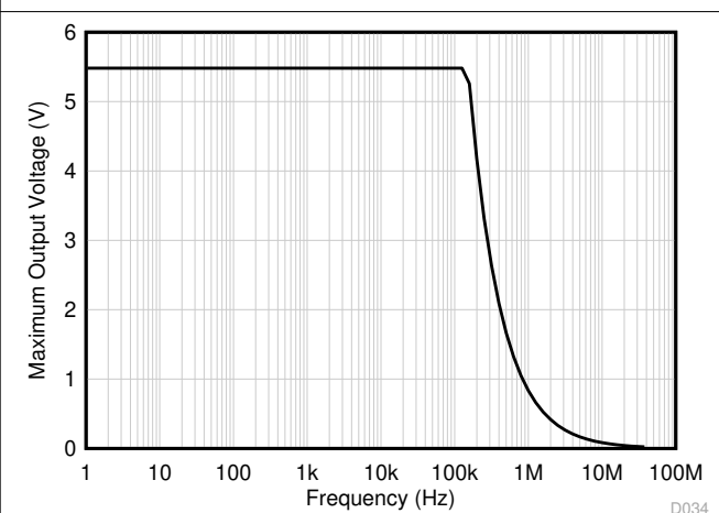
C_L = 10\text{ pF} , Gain = +1, V_S = 5.5\text{ V}
