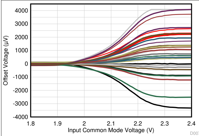
7-45. Offset Voltage vs Common-Mode Voltage (Transition Region)
