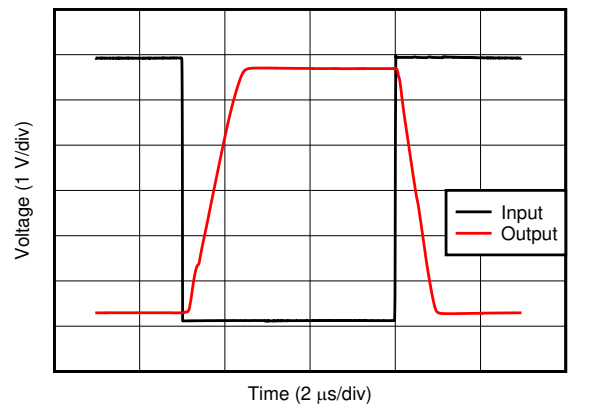
7-30. Overload Recovery
