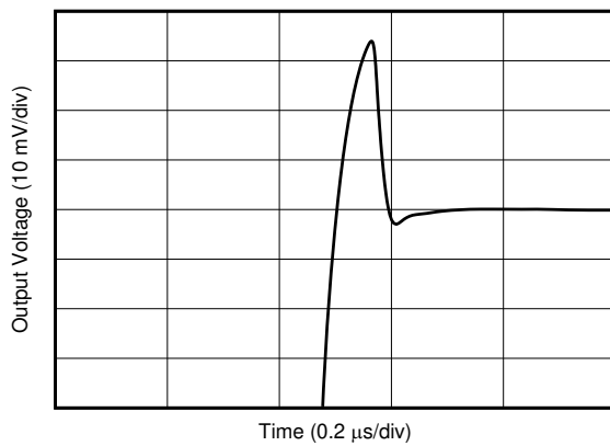
7-31. Small-Signal Step Response
