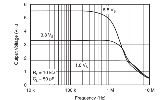
Figure 13. Maximum Output Voltage vs Frequency
