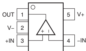
Pin Functions: OPA322-Q1
