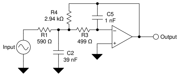
图 47. Typical OPA207 Application Schematic
