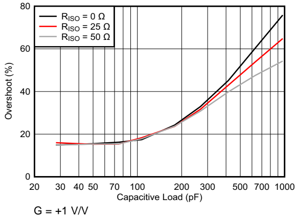
13. Overshoot vs Capacitive Load
