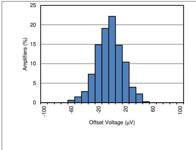
1. Input Referred Offset Voltage Distribution
