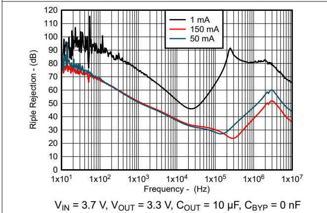
5-17. Ripple Rejection vs Frequency for New Chip
