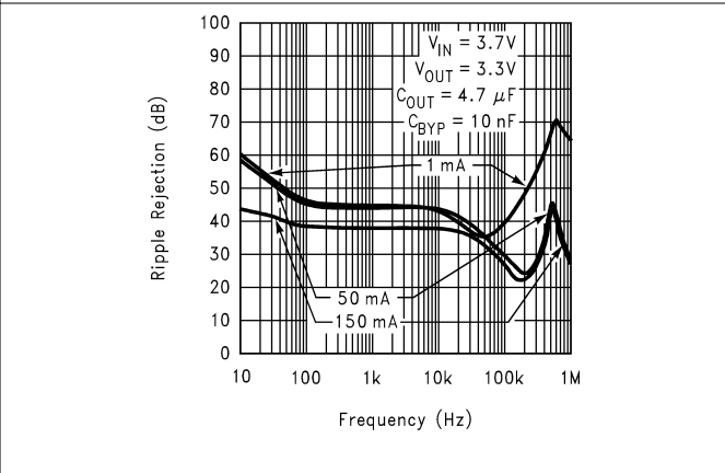
5-18. Ripple Rejection vs Frequency for Legacy Chip
