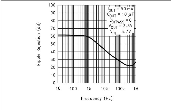
5-15. Ripple Rejection vs Frequency for Legacy Chip
