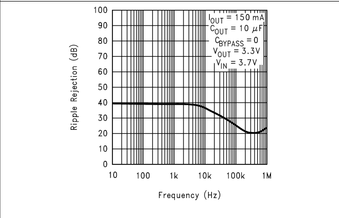
5-16. Ripple Rejection vs Frequency for Legacy Chip
