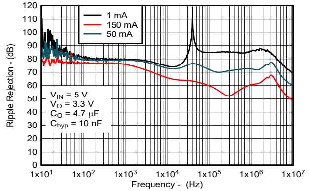
5-20. Ripple Rejection vs Frequency for New Chip
