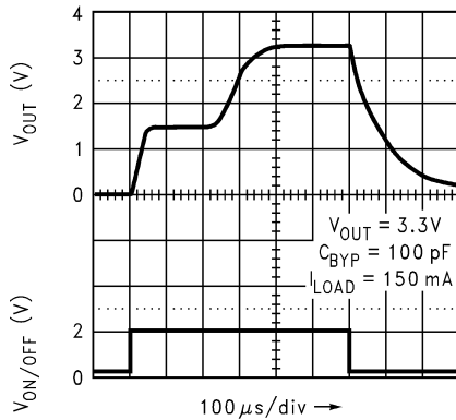
8-21. Turn-On Time for Legacy Chip
