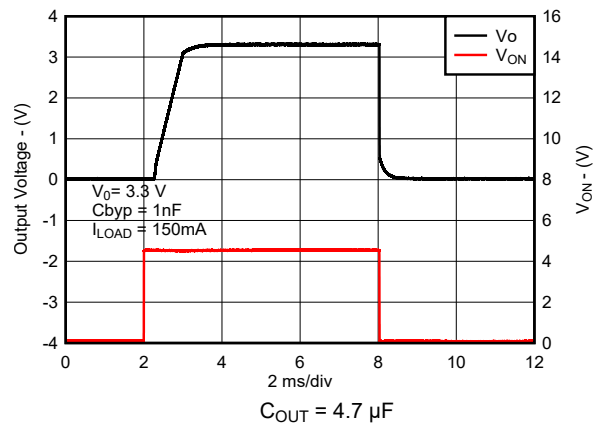
8-26. Turn-On Time for New Chip
