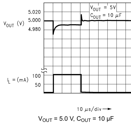
☒ 7-14. Load Transient Response (Legacy Chip)
