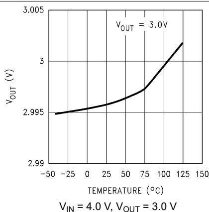
5-3. Output Voltage versus Temperature (Legacy Chip) V_{IN} = 4.0\text{ V} , V_{OUT} = 3.0\text{ V}
