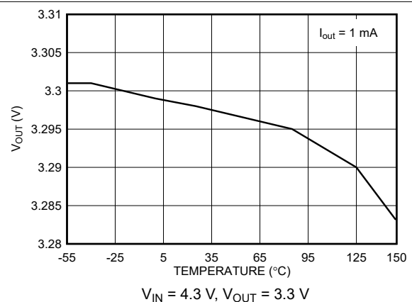
5-4. Output Voltage versus Temperature (New Chip) V_{IN} = 4.3\text{ V} , V_{OUT} = 3.3\text{ V}
