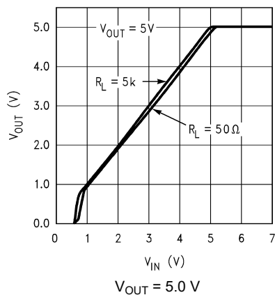
5-5. Output Voltage versus V_{IN} (Legacy Chip) V_{OUT} = 5.0\text{ V}
