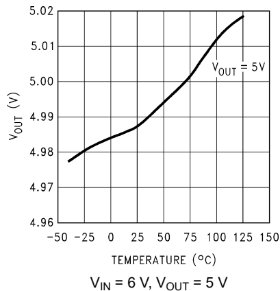
5-1. Output Voltage versus Temperature (Legacy Chip) V_{IN} = 6\text{ V} , V_{OUT} = 5\text{ V}
