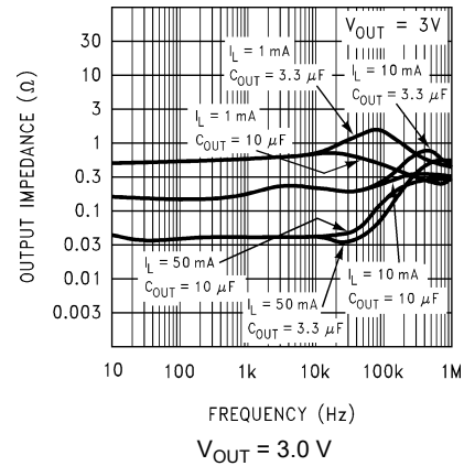
5-40. Output Impedance versus Frequency (Legacy Chip)
