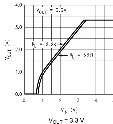
5-6. Output Voltage versus V_{IN} (Legacy Chip) V_{OUT} = 3.3\text{ V}
