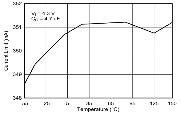
5-36. Instantaneous Short Circuit Current versus Temperature (New Chip)
