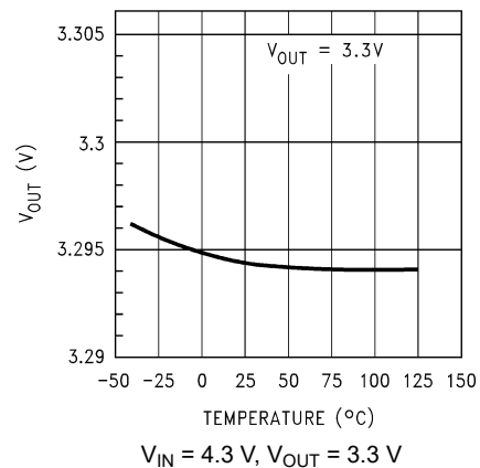
5-2. Output Voltage versus Temperature (Legacy Chip) V_{IN} = 4.3\text{ V} , V_{OUT} = 3.3\text{ V}
