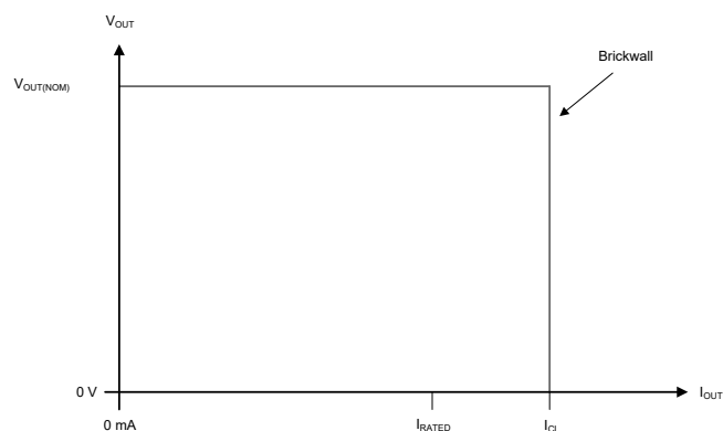
☒ 6-2. Current Limit
