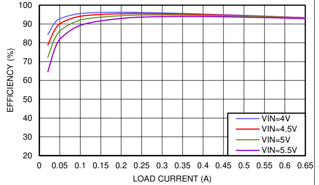
図 8-21. Efficiency V_{OUT} = 3.3\text{ V}
