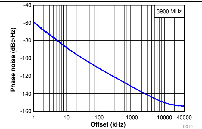
Figure 4. Open-Loop VCO Phase Noise at 3.9 GHz
