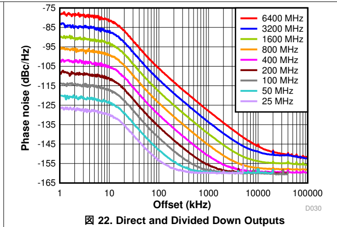
Figure 22. Direct and Divided Down Outputs
