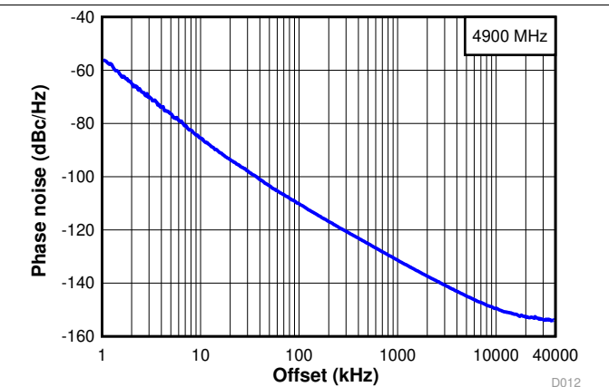
Figure 6. Open-Loop VCO Phase Noise at 4.9 GHz
