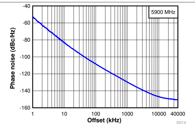
Figure 8. Open-Loop VCO Phase Noise at 5.9 GHz
