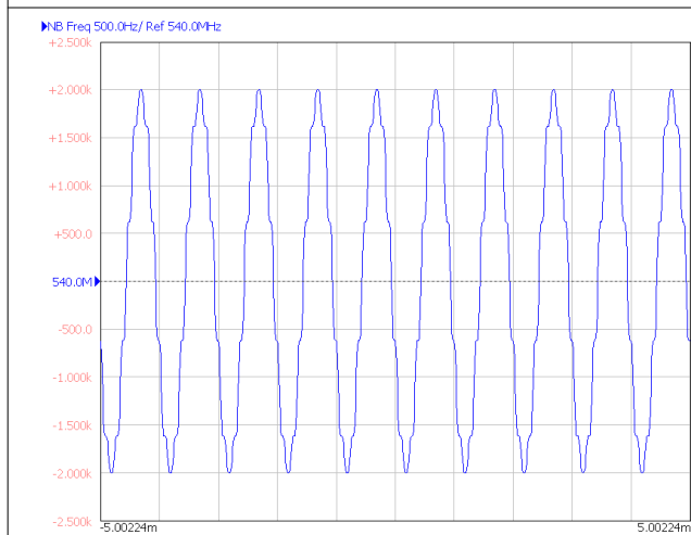
8-34. Simulated FM Modulation (10 Times Over-Sampling)
