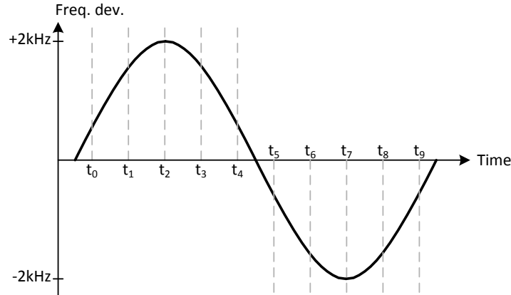
图 8-3. Over-Sampling Modulation Signal
