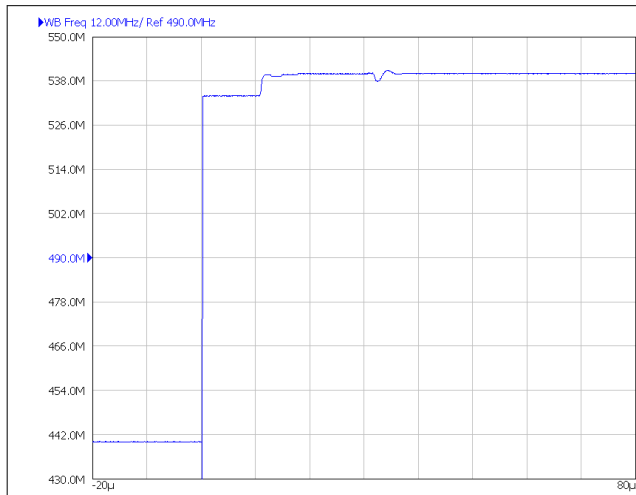
8-30. External VCO to Internal VCO Switching
