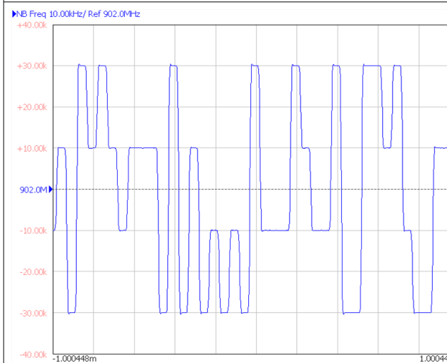
8-20. 4FSK Modulation
