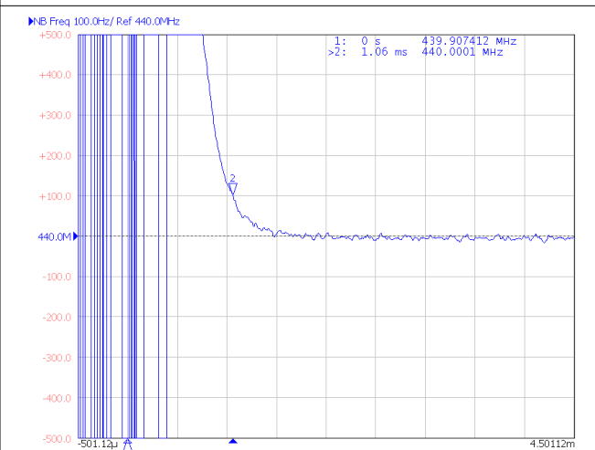
8-33. Internal VCO to External VCO Switching Time
