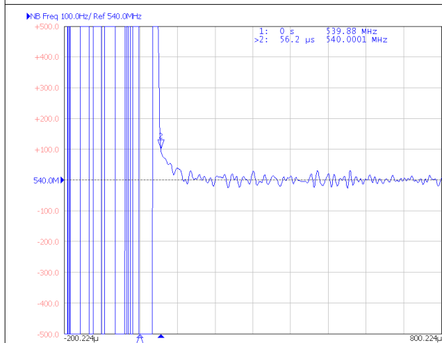
8-32. External VCO to Internal VCO Switching Time
