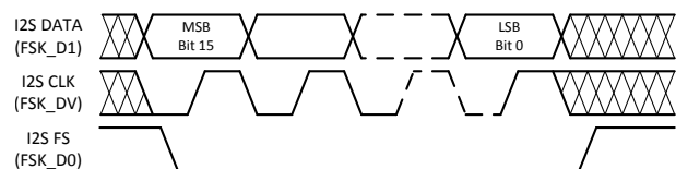
7-5. FSK I2S Mode Timing
