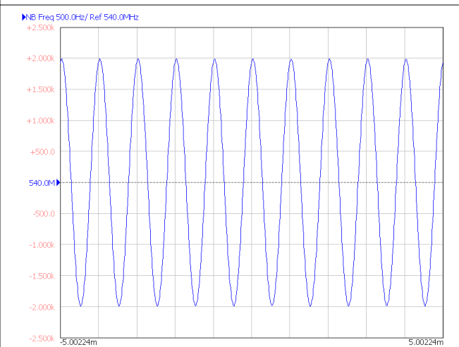
8-35. Simulated FM Modulation (20 Times Over-Sampling)
