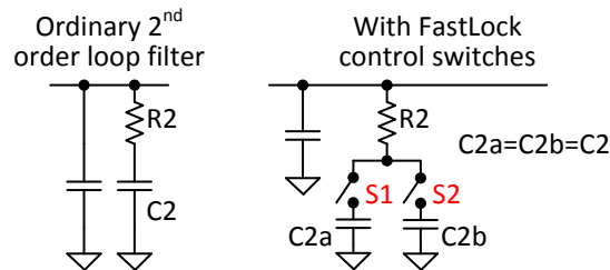
8-7. FastLock With SPST Switches
