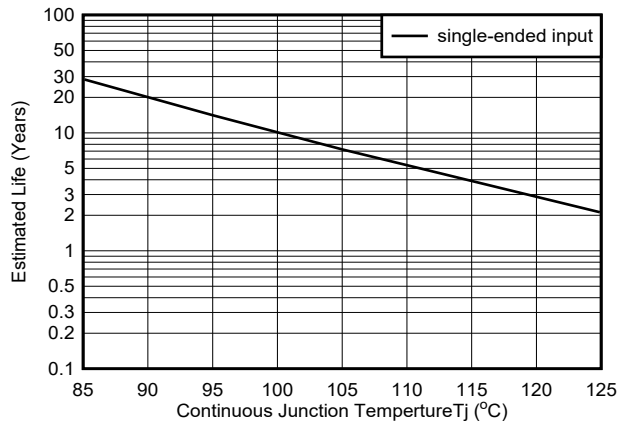
6-14. Lifetime vs. Temperature
