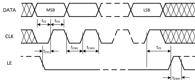
6-1. MICROWIRE Timing Diagram
