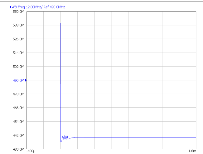
8-31. Internal VCO to External VCO Switching
