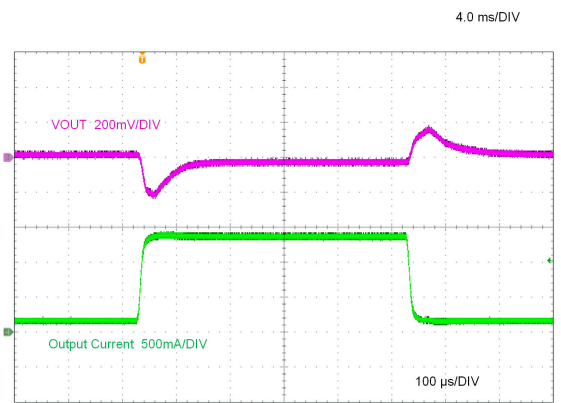
LMR38015-Q1 V_{OUT} = 5V 400kHz (AC 結合)
