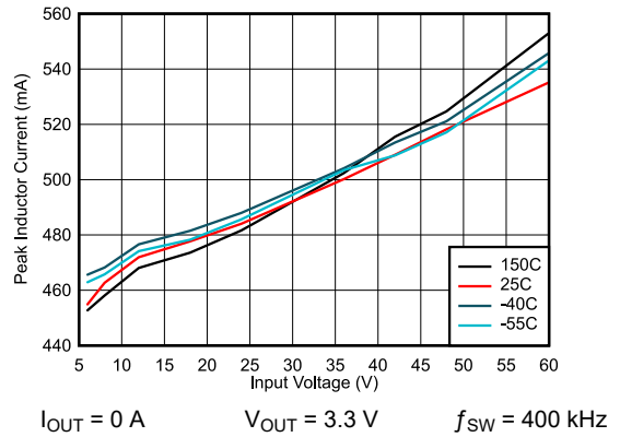
8-6. I_{PEAK-MIN}
