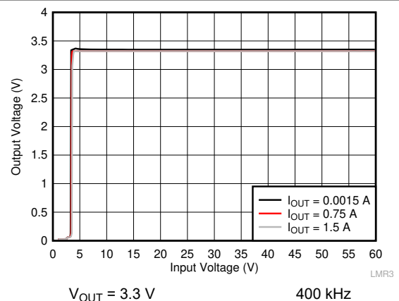
10-9. Line Regulation
