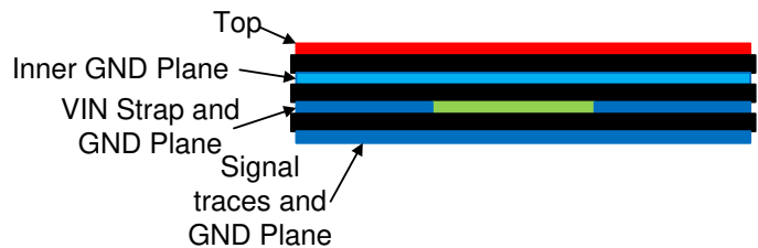
12-2. Example Layout
