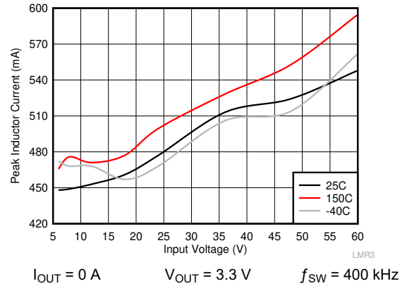
8-6. I_{PEAK-MIN}
