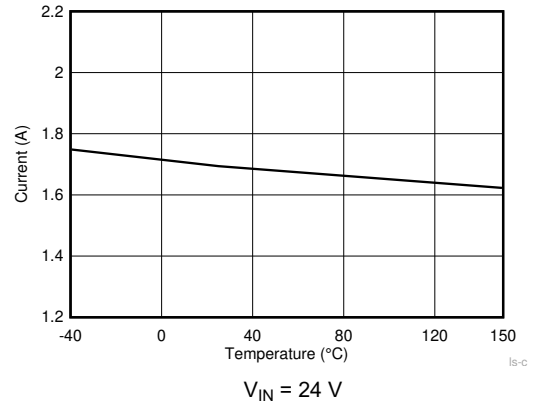
8-4. Low Side Current Limit
