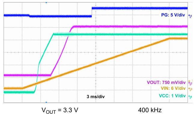
10-15. Start-Up Waveform
