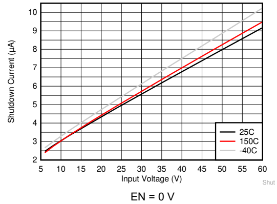
8-2. Shutdown Supply Current
