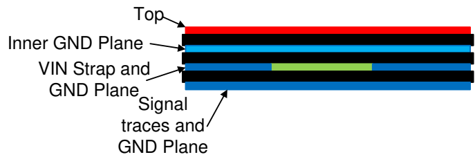
10-3. Example Layout for 400kHz, Adjustable Output
