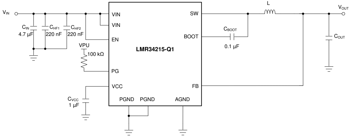
图 9-2. Example Applications Circuit (Fixed 5-V Output)
