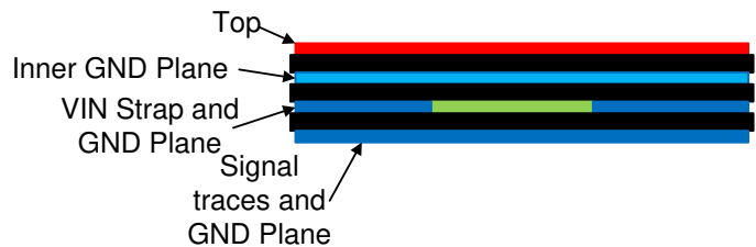
FIG 10-2. Example Layout for Fixed Output
