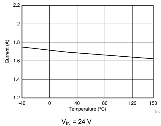
7-4. Low Side Current Limit
