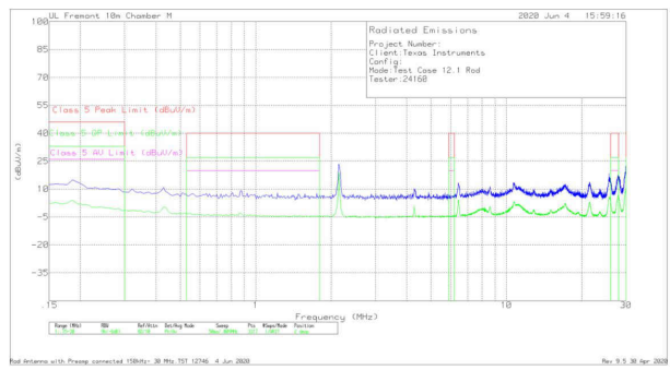
V_{OUT} = 5V F_{SW} = 2.1MHz I_{OUT} = 4A 測定周波数: 150kHz~30MHz
