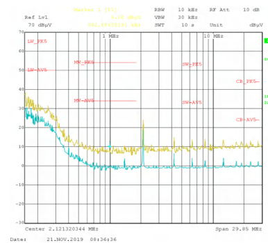
F_{SW} = 2100kHz V_{OUT} = 5V I_{OUT} = 5A 測定周波数: 150kHz~300MHz
