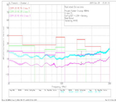
V_{OUT} = 5V F_{SW} = 400kHz I_{OUT} = 5A 測定周波数: 30MHz~300MHz
