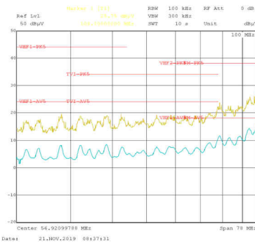
V_{OUT} = 5V F_{SW} = 2100kHz I_{OUT} = 5A 測定周波数: 30MHz~108MHz
