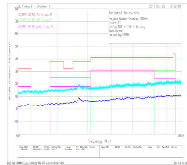
V_{OUT} = 5V F_{SW} = 400kHz I_{OUT} = 5A 測定周波数: 300MHz~1GHz
