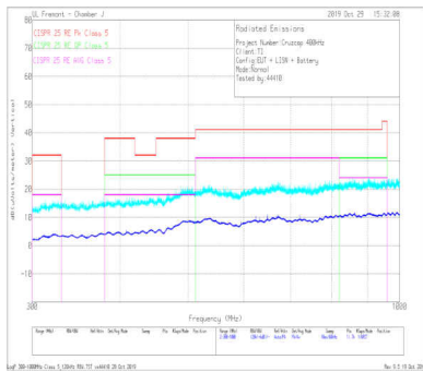
V_{OUT} = 5V F_{SW} = 400kHz I_{OUT} = 5A 測定周波数: 300MHz~1GHz
