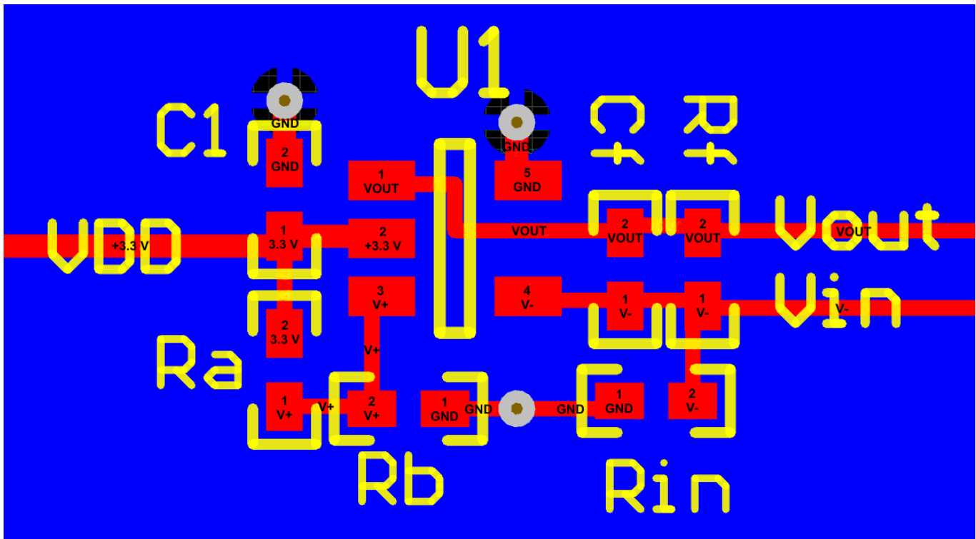
☒ 7-5. LMC7101 Example Layout
