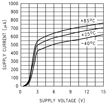
5-23. Supply Current vs Supply Voltage
