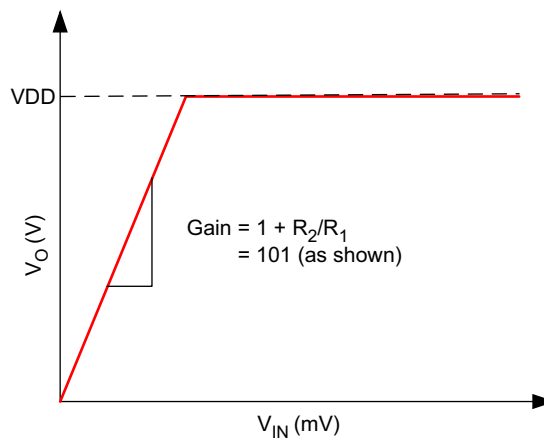
☒ 7-4. Output Response
