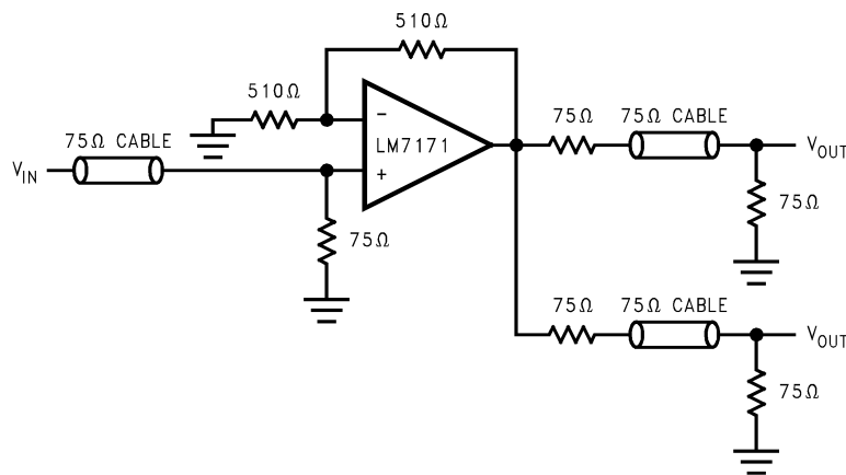
図 6-5. Video Line Driver
