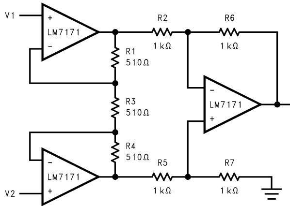
6-2. Fast Instrumentation Amplifier
