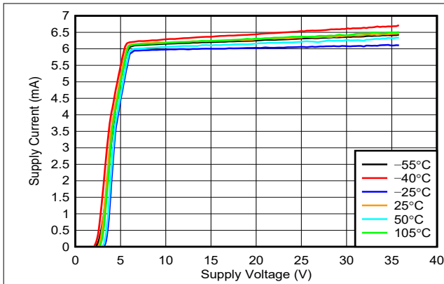
図 5-1. Supply Current vs Supply Voltage
