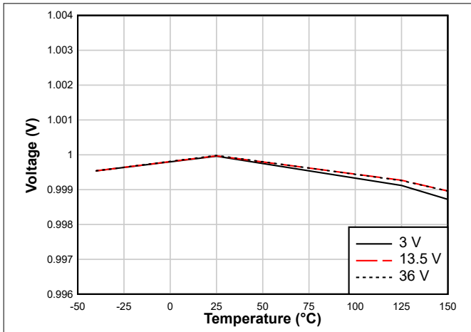
7-1. Feedback Voltage
