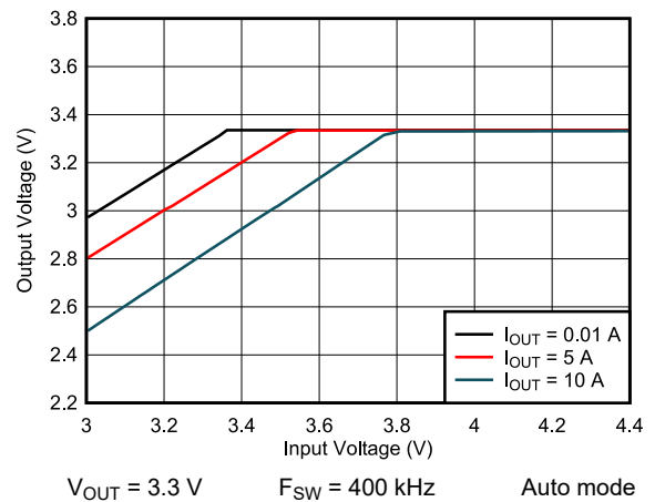
9-22. Dropout
