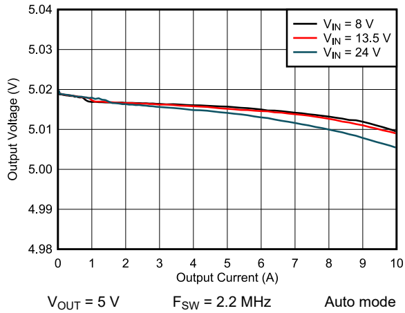
9-17. Load and Line Regulation
