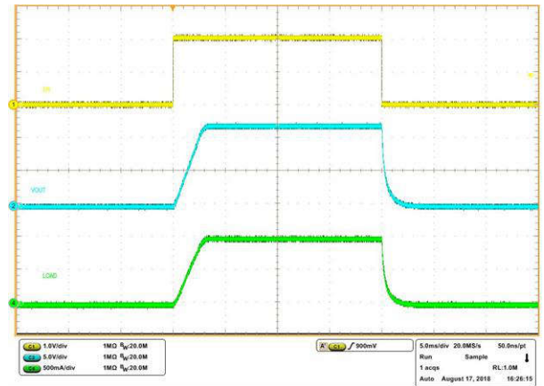
7-9. Full-Load Start-up and Shutdown with EN/UVLO
