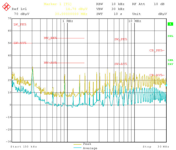
7-14. No-Load Switching
