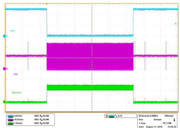
7-11. Short Circuit Applied
