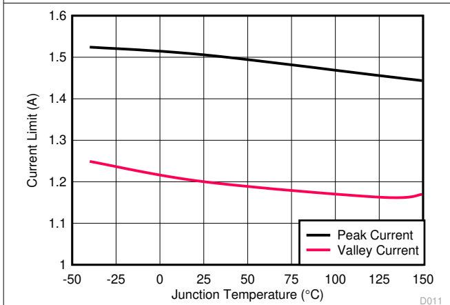
5-9. Peak and Valley Current Limit versus Temperature
