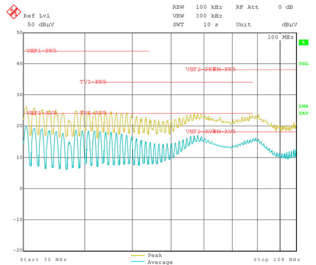
7-15. Full-Load Switching
