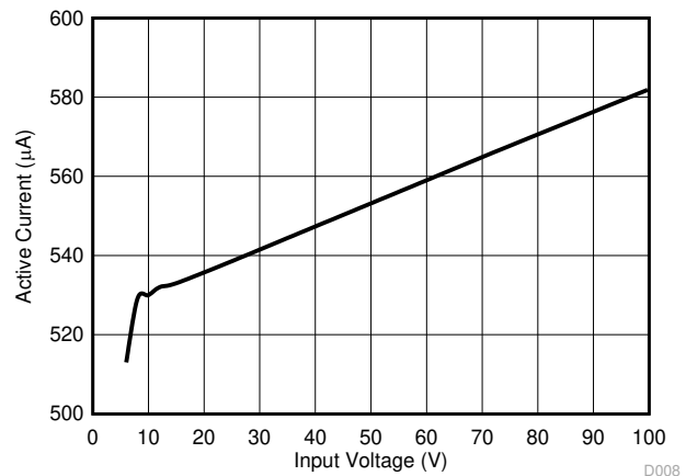
図 5-6. V_{IN} Active Current versus Input Voltage
