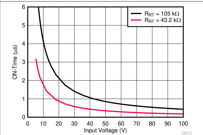
5-10. COT On-Time versus V_{IN}
