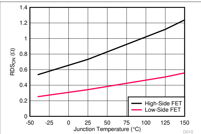
5-8. MOSFETs On-State Resistance versus Temperature
