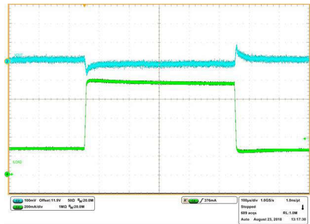
V_{IN} = 24\text{ V} I_{OUT} = 0.25\text{ A to } 1\text{ A at } 0.1\text{ }\mu\text{s}
