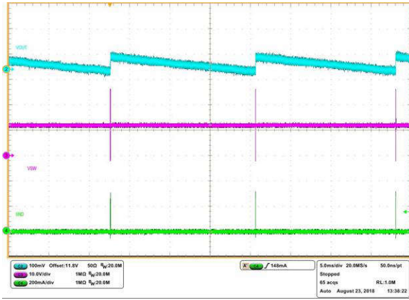
7-14. No-Load Switching
