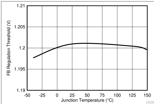
5-7. Feedback Comparator Threshold versus Temperature
