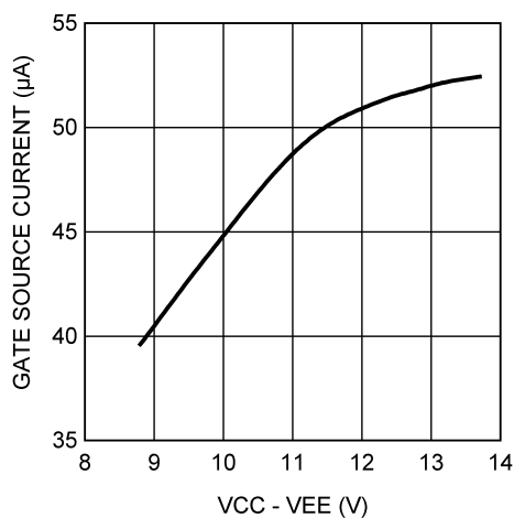
7-6. GATE Source Current vs Operating Voltage
