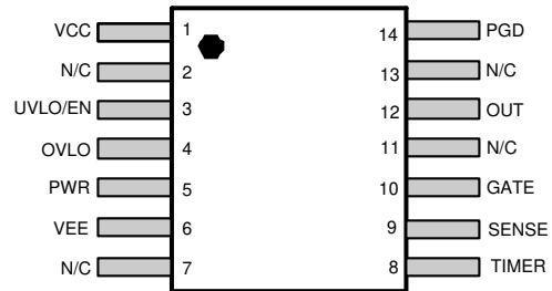
6-2. 14-Lead SOIC Top View
