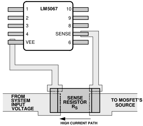
9-2. Sense Resistor Connections
