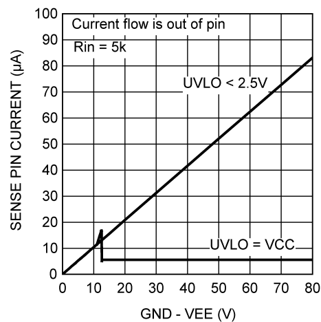
7-4. SENSE Pin Current vs System Voltage
