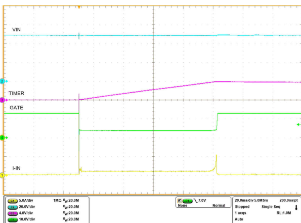
9-22. Short Circuit and Release
