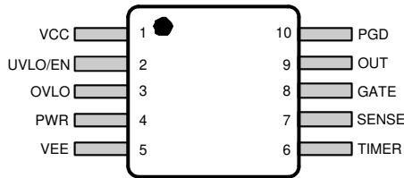
6-1. 10-Lead VSSOP Top View
