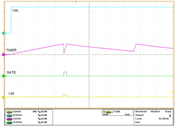
9-19. Power Into Short
