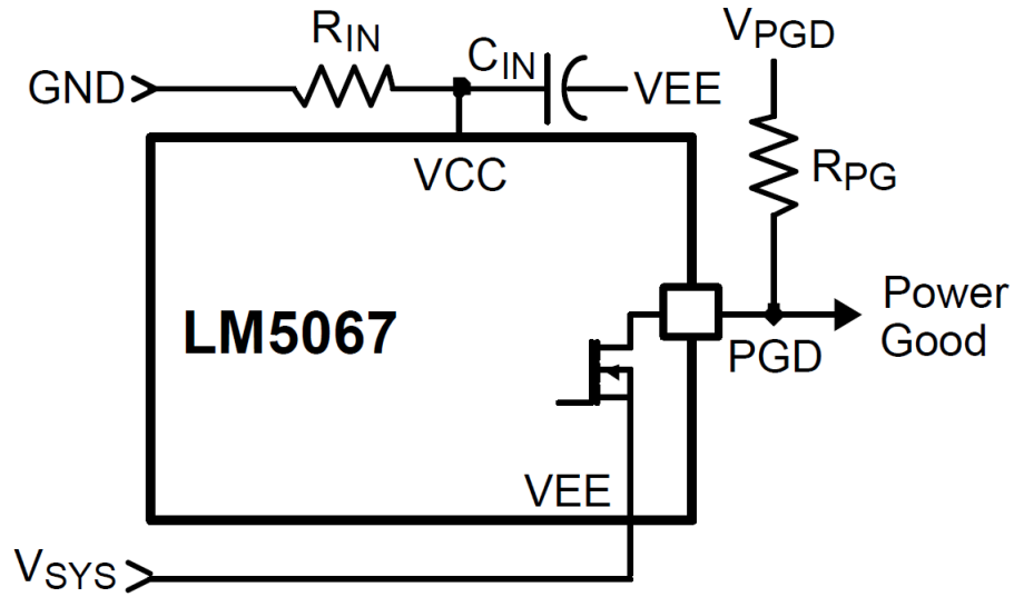
9-12. Power Good Output
