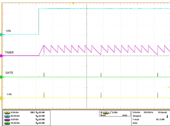
9-20. Power Into Short Retry Zoomed Out
