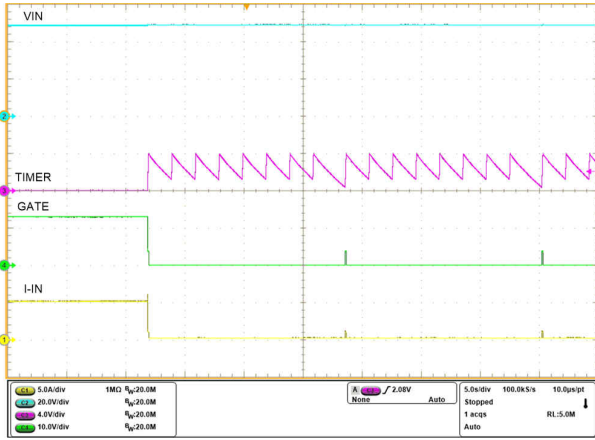
9-18. Overload With Retry
