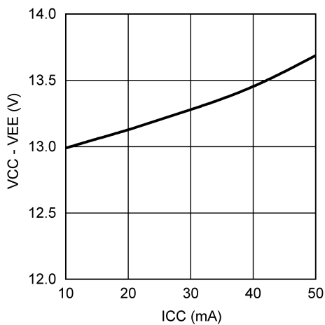
7-3. Operating Voltage vs ICC
