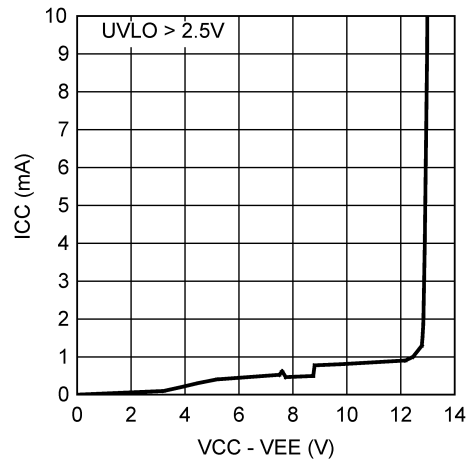
7-2. ICC vs Operating Voltage - Enabled
