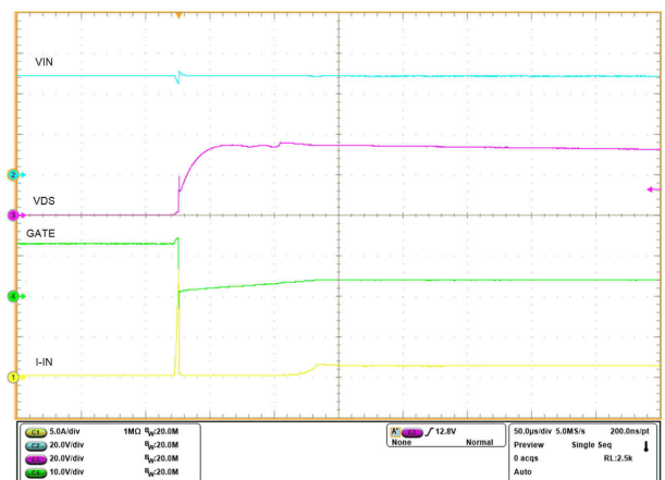
9-23. Short Circuit Zoomed In
