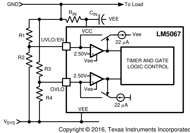
9-7. Programming the Four Thresholds
