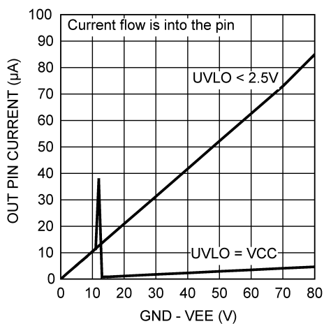
7-5. OUT Pin Current vs System Voltage
