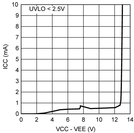
7-1. ICC vs Operating Voltage - Disabled
