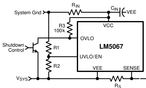
☒ 8-7. Shutdown/Enable Using the OVLO Pin
