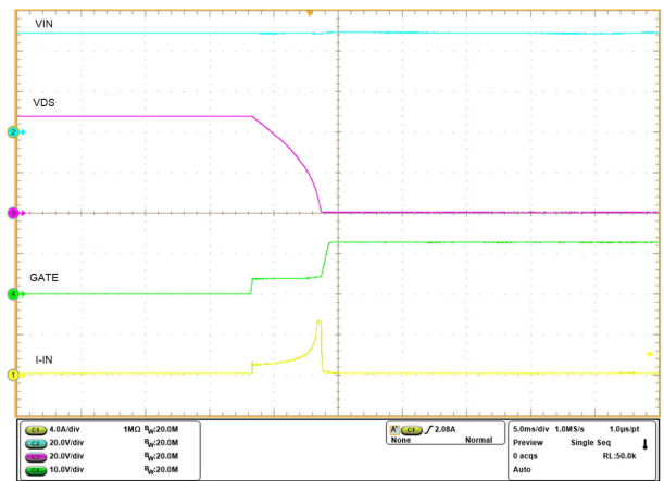
9-21. Power Limited Startup
