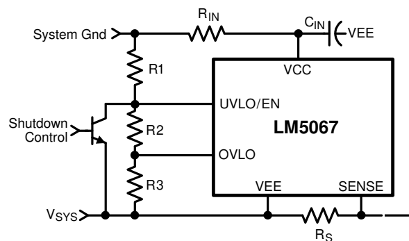
☒ 8-6. Shutdown/Enable Using the UVLO/EN Pin
