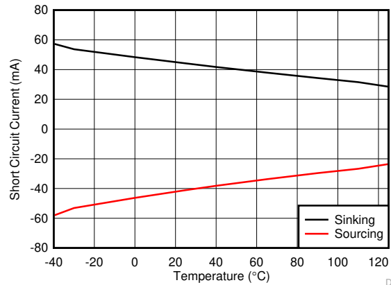
6-27. Short-Circuit Current vs Temperature
