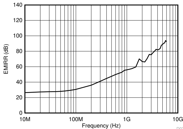
6-28. Electromagnetic Interference Rejection Ratio Referred to Noninverting Input (EMIRR+) vs Frequency
