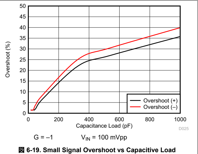
Figure 6-19. Small Signal Overshoot vs Capacitive Load
