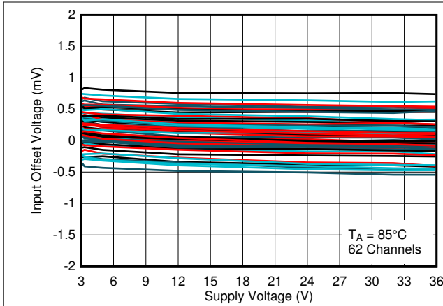
7-13. Input Offset Voltage vs. Supply Voltage at 85°C
