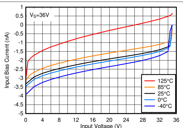
7-18. Input Bias Current vs. Input Voltage at 36V
