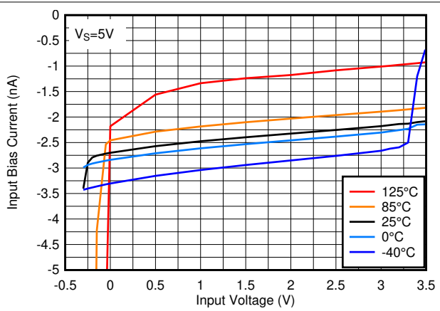
7-16. Input Bias Current vs. Input Voltage at 5V
