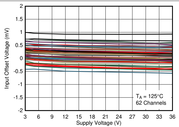
7-14. Input Offset Voltage vs. Supply Voltage at 125°C
