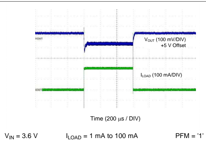
Figure 14. PFM Load Step
