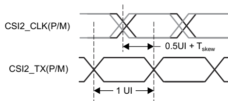
図 8-12. Clock and Data Timing in HS Transmission
