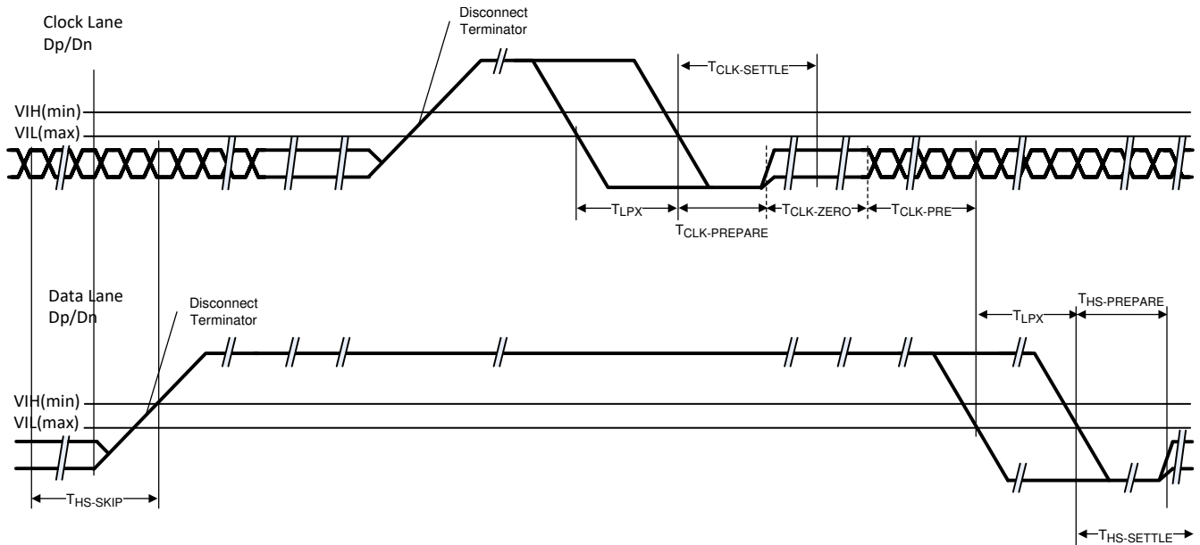
8-13. High-Speed Data Transmission Burst
