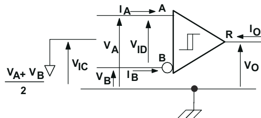
7-7. Receiver Voltage and Current Definitions
