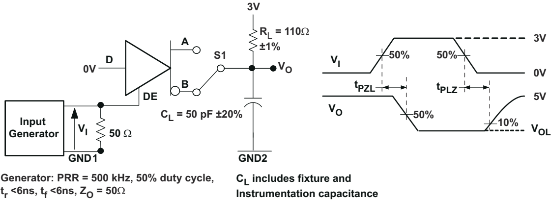
7-6. Driver Low-Level Output Enable and Disable Time Test Circuit and Voltage Waveform
