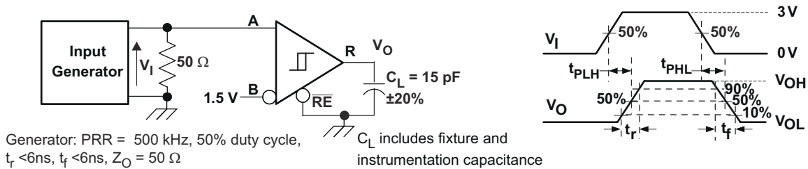
7-8. Receiver Switching Test Circuit and Waveforms
