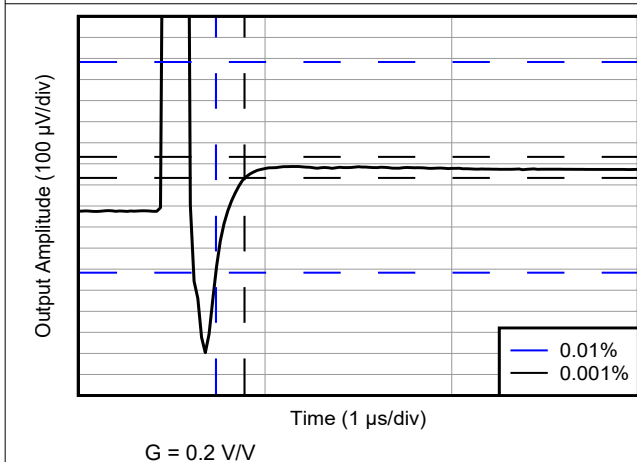
7-53. Settling Time for G = 0.2\text{ V/V}
