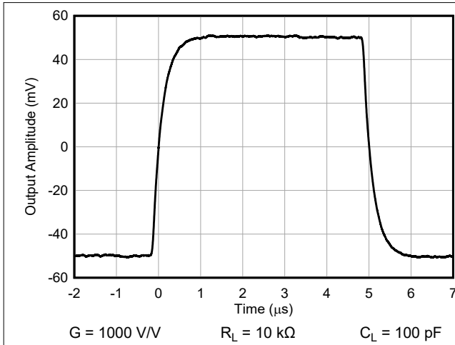
7-49. Small-Signal Response for G = 1000\text{ V/V}
