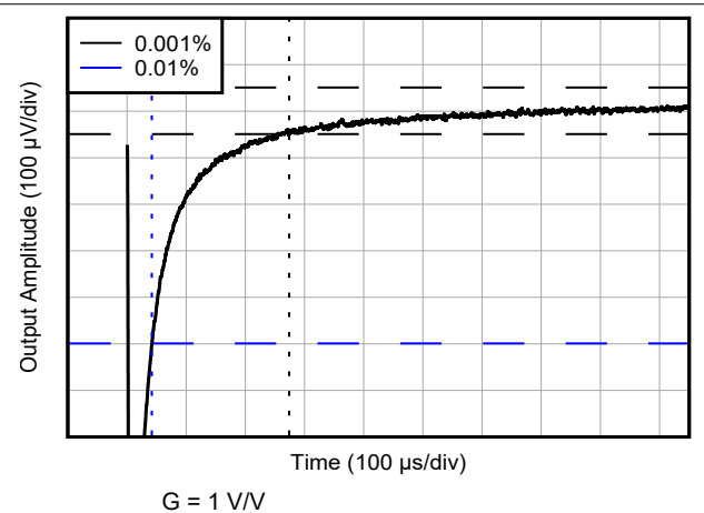
7-54. Settling Time for G = 1\text{ V/V}
