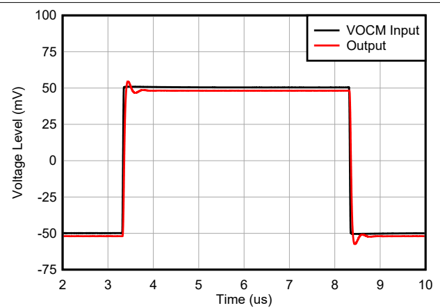
7-50. Small-Signal Response of VOCM Amplifier
