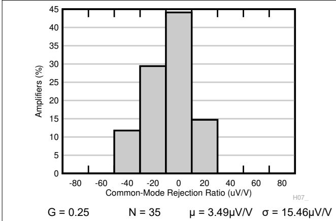
Figure 6-9. Typical Distribution of Output Referred CMRR
