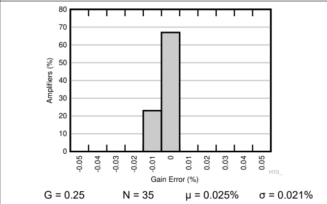
Figure 6-12. Typical Distribution of Gain Error
