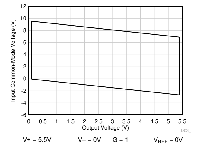
6-68. Input Common-Mode Voltage vs Output Voltage (High CMRR Region)
