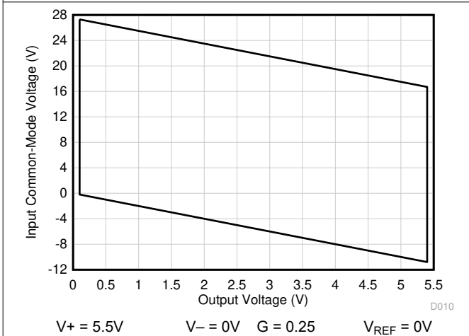
6-69. Input Common-Mode Voltage vs Output Voltage (Rail-to-Rail CMRR Region)
