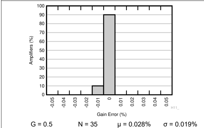
Figure 6-11. Typical Distribution of Gain Error
