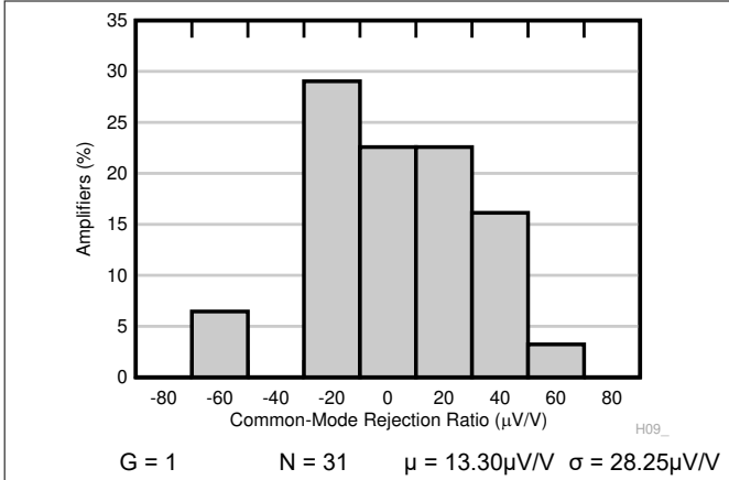
Figure 6-7. Typical Distribution of Output Referred CMRR
