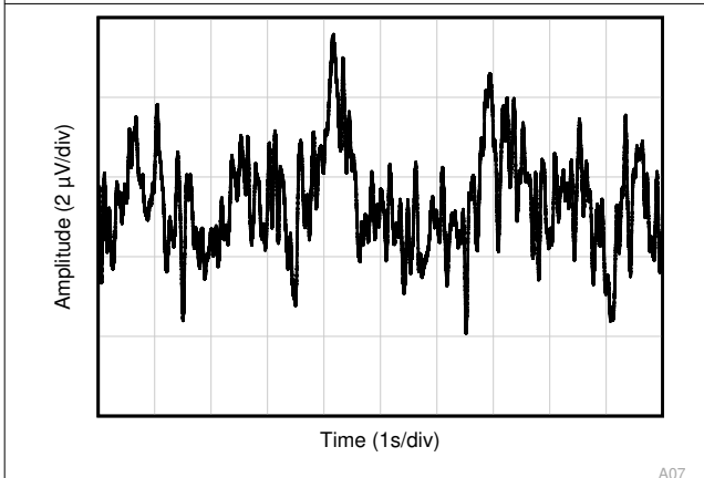
6-41. Output Referred 0.1 Hz to 10 Hz Voltage Noise in Time Domain
