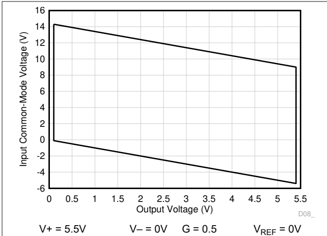
6-67. Input Common-Mode Voltage vs Output Voltage (High CMRR Region)
