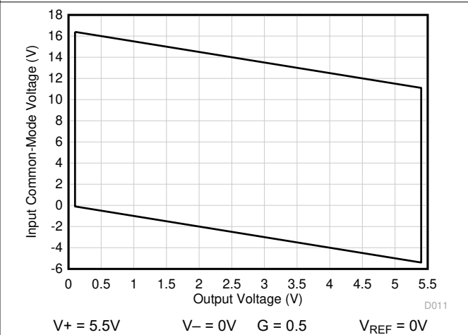
6-70. Input Common-Mode Voltage vs Output Voltage (Rail-to-Rail CMRR Region)
