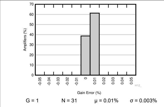
Figure 6-10. Typical Distribution of Gain Error
