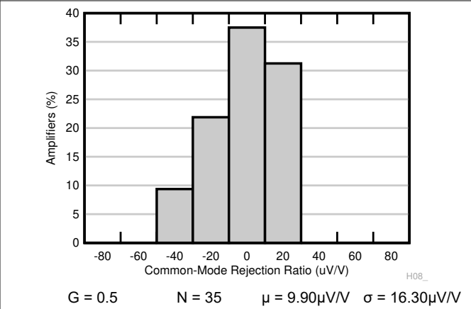
Figure 6-8. Typical Distribution of Output Referred CMRR
