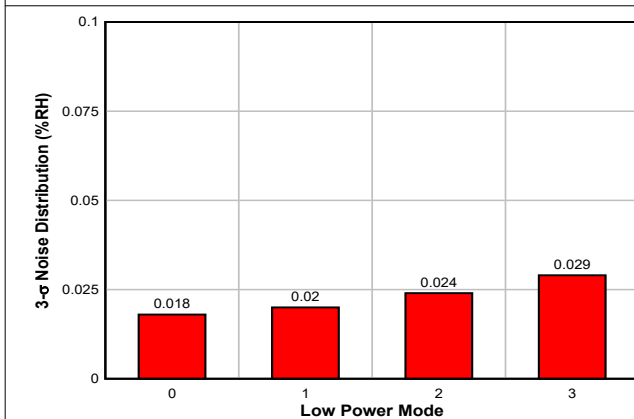
Figure 7-6. Typical RH Noise Across Low Power Modes
