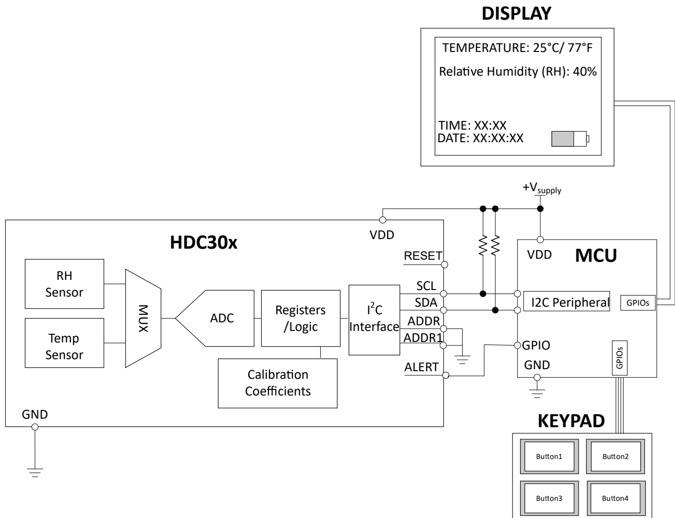
9-1. Typical Application Schematic HVAC
