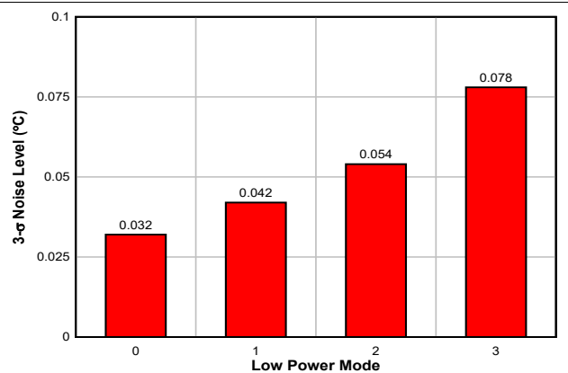
Figure 6-7. Typical Temperature Noise Across Low Power Modes
