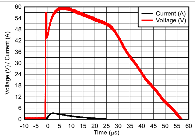
图 5-4. 8/20 μs Surge Response
