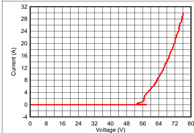
图 5-3. Positive TLP Curve
