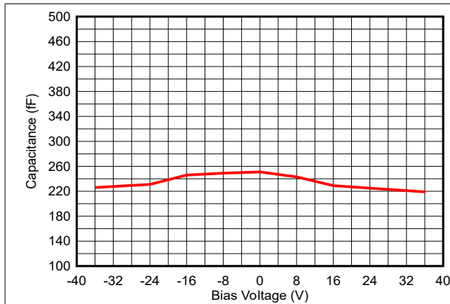
图 5-1. Bias Voltage vs Capacitance
