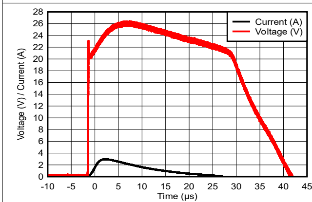
図 5-5. 8/20 \mu s Surge Response
