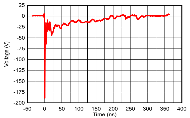
図 5-6. -8kV Clamped IEC Waveform
