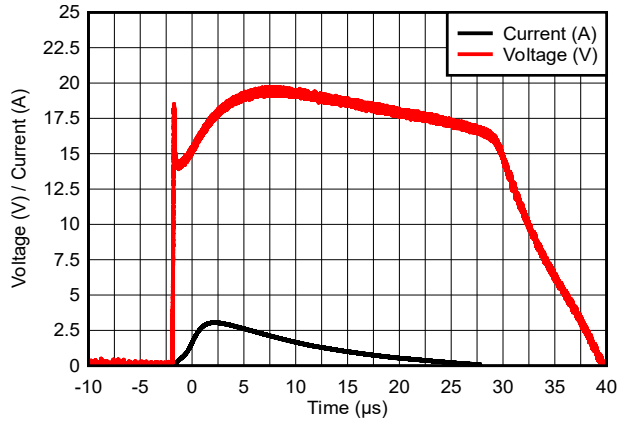
5-7. 8/20 μs Surge Response
