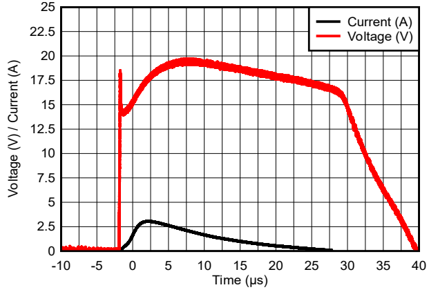
5-7. 8/20 μs Surge Response
