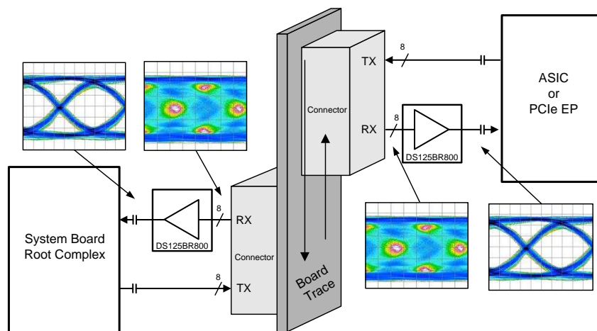
Figure 9. Typical Application
