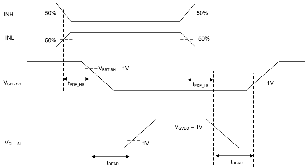
6-2. Gate Driver Dead Timing Insertion (INH and INL monitor mode)
