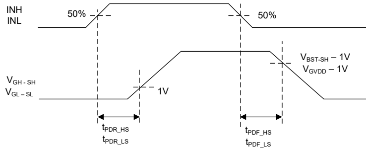
6-1. Gate Driver Propagation Delay Timing Diagram
