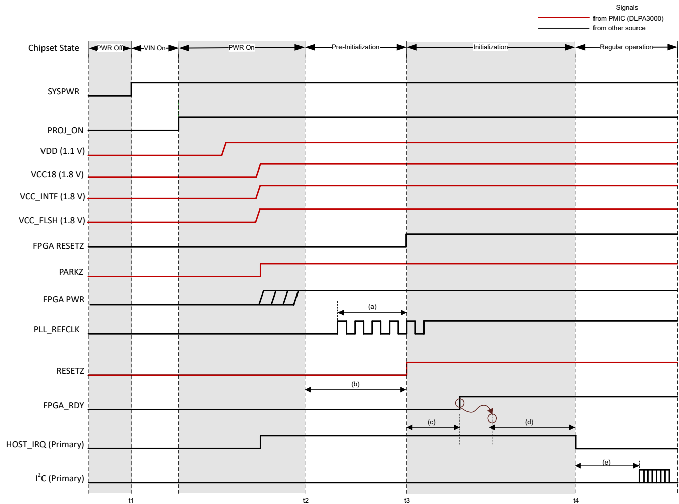
9-1. DLPC3437 Power-Up Timing
