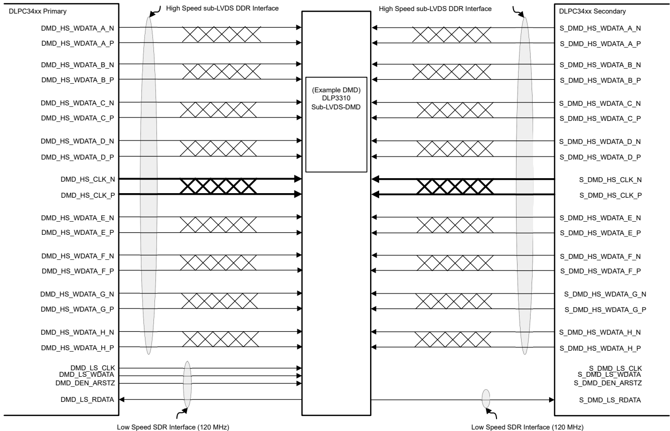
图 7-12. DLP3310 (.33 1080p) DMD Interface Example (Option 1 and 2)
