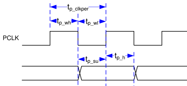
6-8. Parallel Interface General Timing
