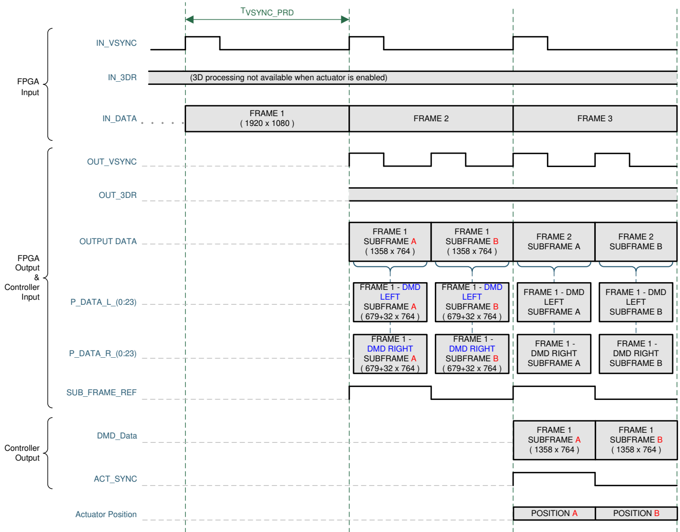
7-2. DLPC3437 2D Actuator Frame and Signal Timing
