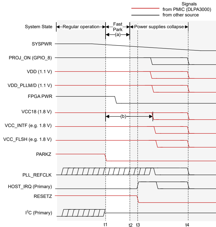
9-3. DLPC3437 Fast Power-Down
