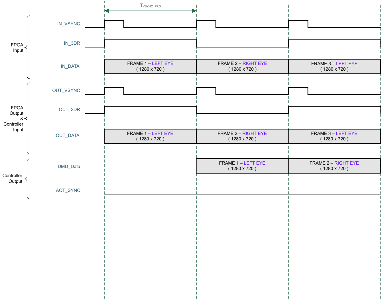
☒ 7-3. DLPC3437 3D Frame and Signal Timing
