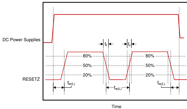
図 5-6. Power-Up and Power-Down RESETZ Timing
