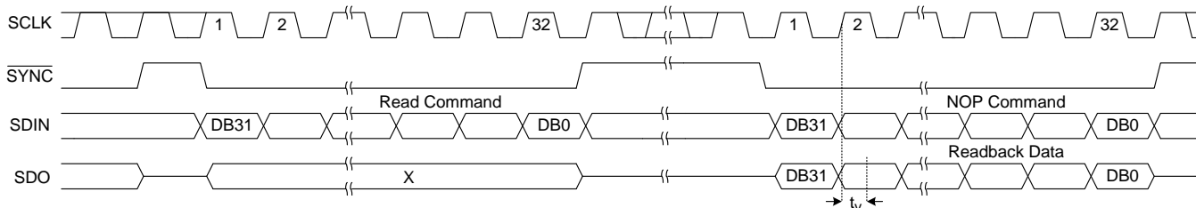
Figure 54. Read-Back Operation
