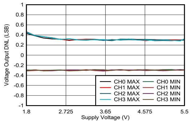
6-11. Voltage Output DNL vs Supply Voltage
