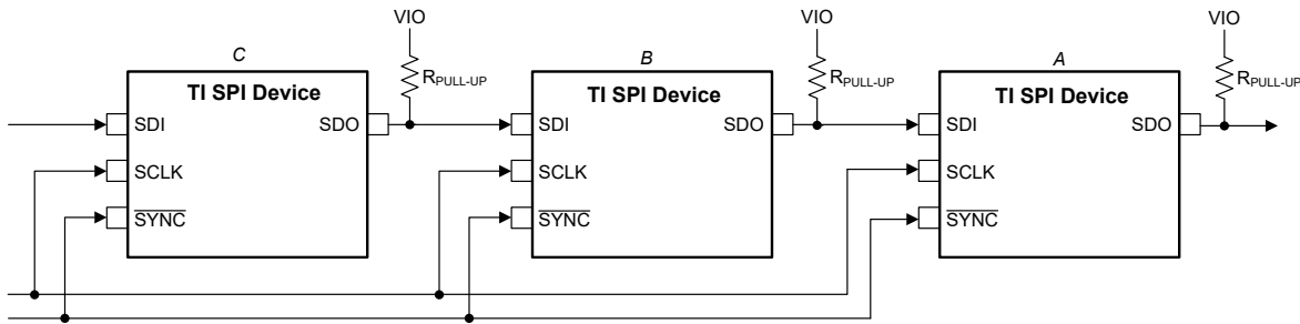
図 6-16. SPI Daisy-Chain Connection
