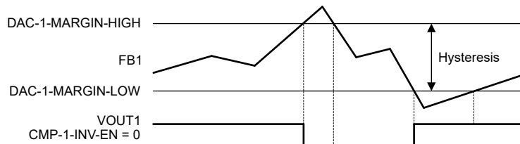
図 6-4. Programmable Hysteresis Without Latching Output
