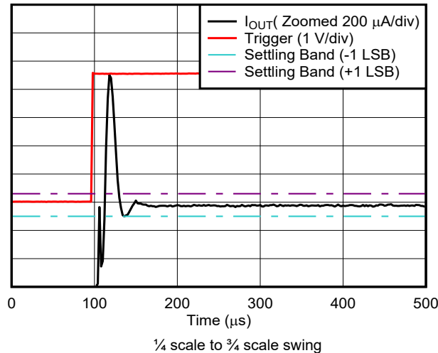
5-39. Current Output Setting Time, Rising Edge
