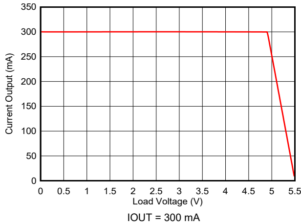
5-37. Current Output vs Load Voltage
