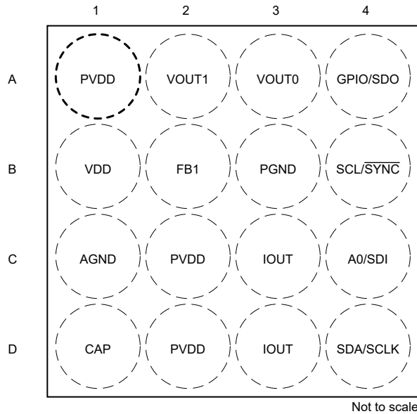
図 4-1. DAC532A3W: YBH (16-pin DSBGA) Package, Top View
