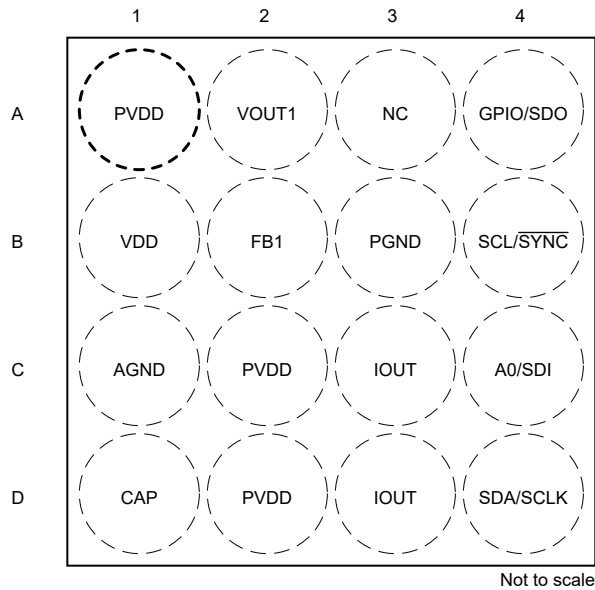
図 4-2. DAC530A2W: YBH (16-pin DSBGA) Package, Top View
