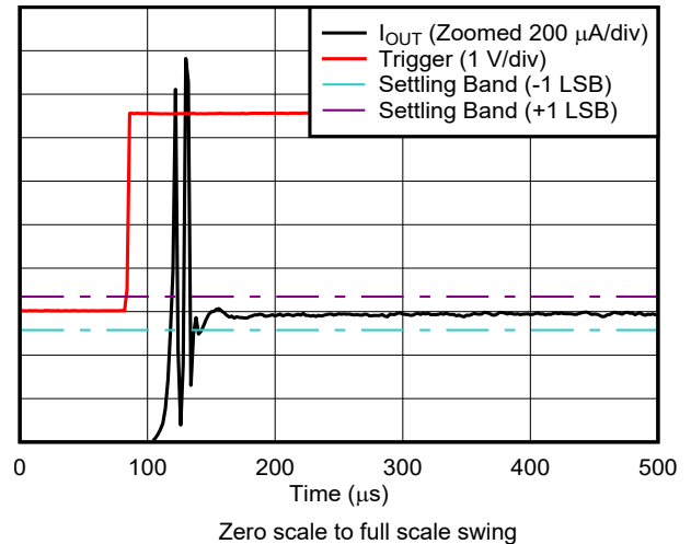
5-40. Current Output Setting Time, Rising Edge
