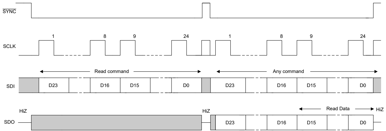
図 6-15. SPI Read Cycle
