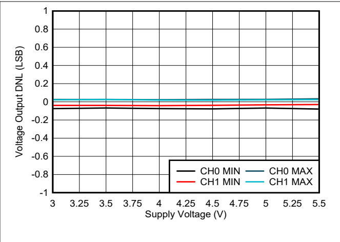
5-11. Voltage Output DNL vs Supply Voltage
