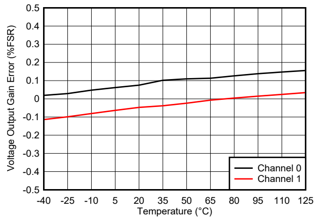
图 5-17. Voltage Output Gain Error vs Temperature
