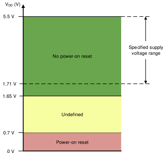
图 6-13. Threshold Levels for V_{DD} POR Circuit
