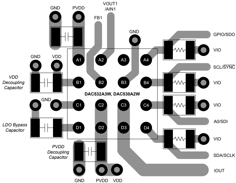
8-4. Layout Example
