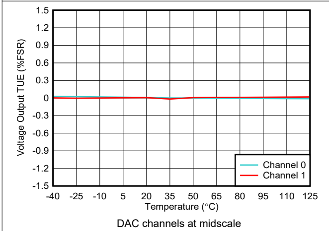
5-14. Voltage Output TUE vs Temperature
