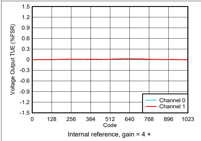
5-12. Voltage Output TUE vs Digital Input Code
