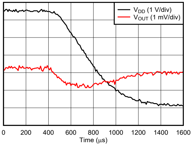
5-24. Voltage Output Power-Off Glitch
