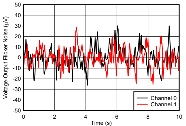
5-27. Voltage Output Flicker Noise
