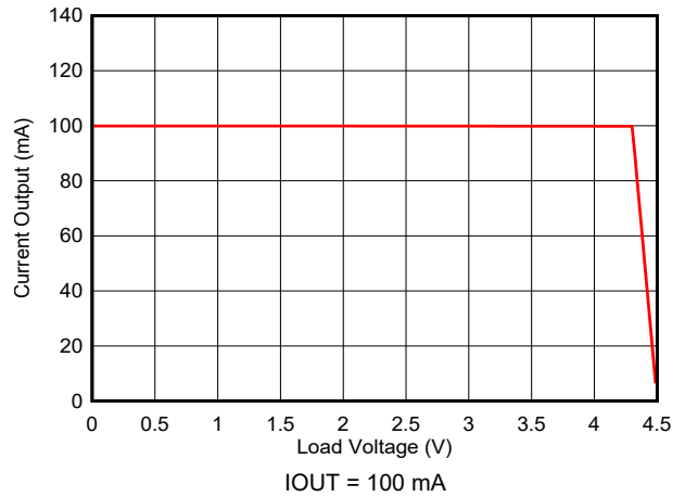
5-38. Current Output vs Load Voltage
