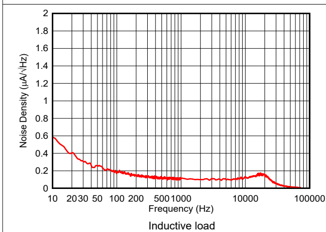
Figure 5-45. Current Output Noise Density
