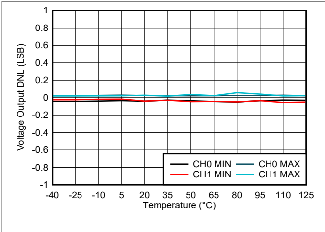
5-10. Voltage Output DNL vs Temperature
