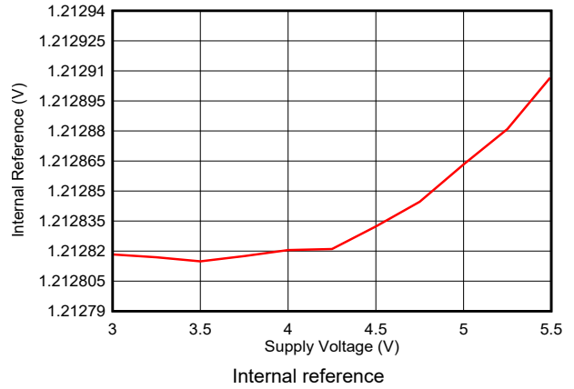
Figure 5-54. Internal Reference vs Supply Voltage
