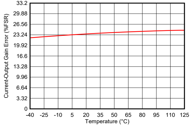
5-36. Current Output Gain Error vs Temperature
