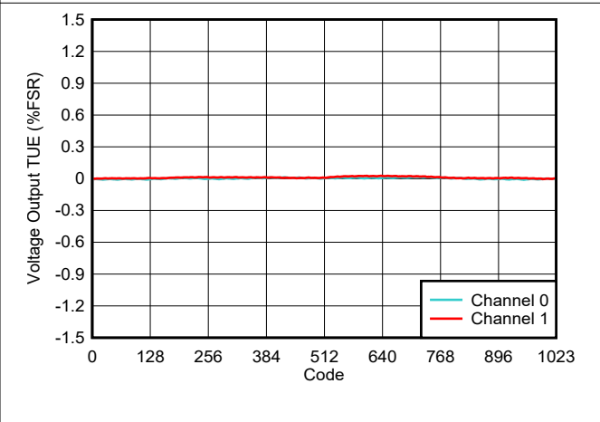
5-13. Voltage Output TUE vs Digital Input Code
