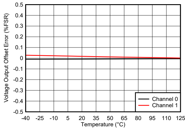
图 5-16. Voltage Output Offset Error vs Temperature
