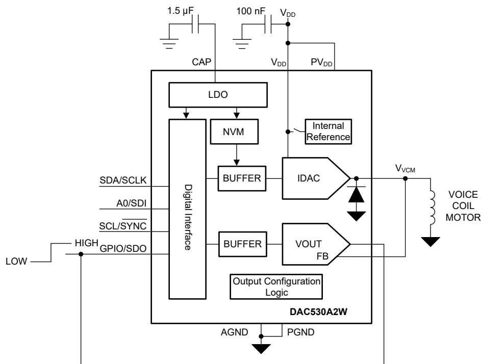
図 8-1. Voice Coil Motor Control
