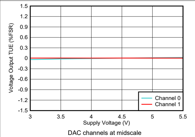
5-15. Voltage Output TUE vs Supply Voltage
