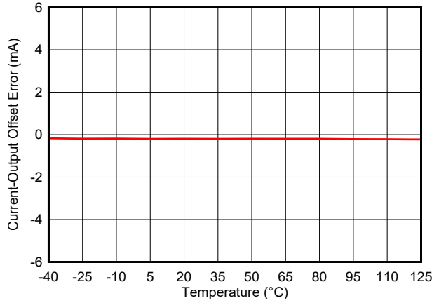
5-35. Current Output Offset Error vs Temperature
