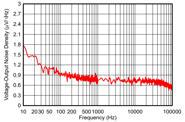
5-25. Voltage Output Noise Density
