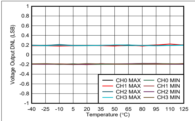
6-10. Voltage Output DNL vs Temperature
