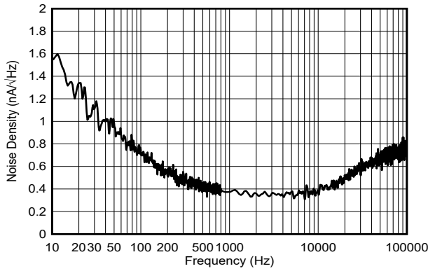
6-49. Current Output Noise Density
