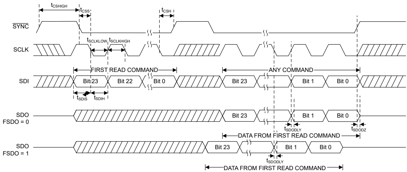
6-3. SPI Read Timing Diagram
