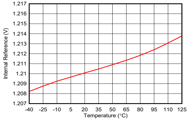
6-54. Internal Reference vs Temperature
