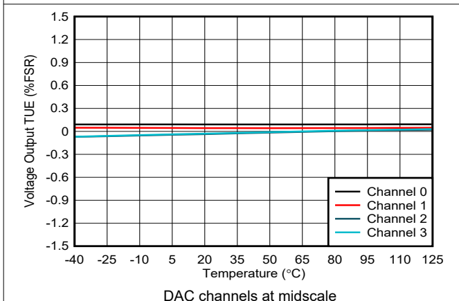
6-14. Voltage Output TUE vs Temperature
