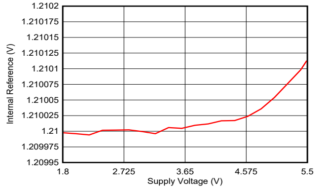
6-55. Internal Reference vs Supply Voltage
