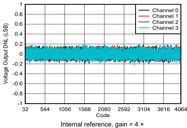
6-8. Voltage Output DNL vs Digital Input Code
