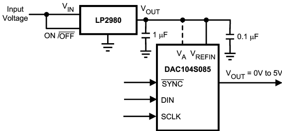
FIGURE 8. Using the LP2980 regulator
