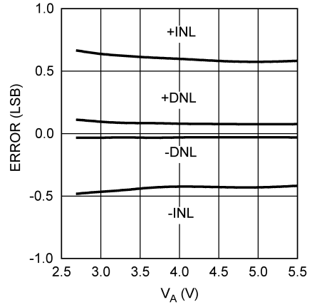
INL/DNL vs V_A
