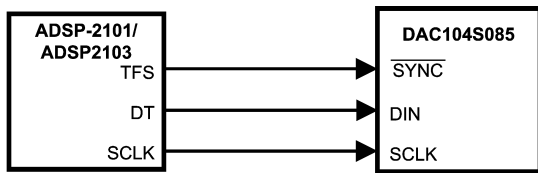
FIGURE 10. ADSP-2101/2103 Interface
