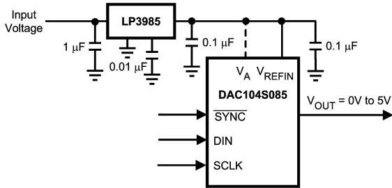
FIGURE 7. Using the LP3985 regulator
