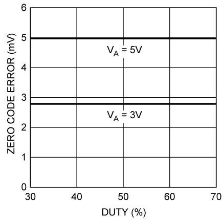
Zero Code Error vs. Clock Duty Cycle
