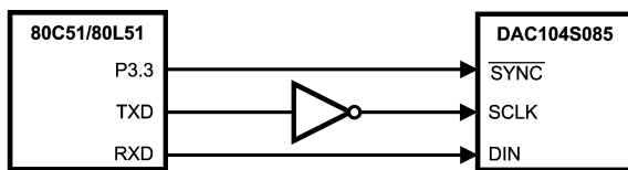
FIGURE 11. 80C51/80L51 Interface
