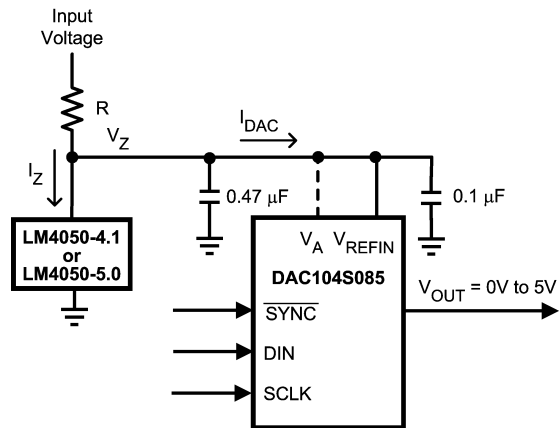
FIGURE 6. The LM4050 as a power supply
