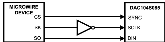
FIGURE 13. Microwire Interface
