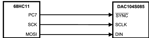
FIGURE 12. 68HC11 Interface
