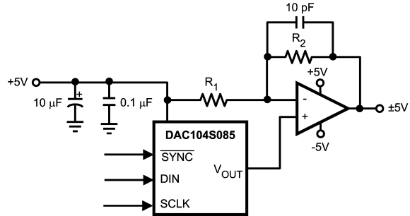
FIGURE 9. Bipolar Operation
