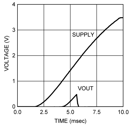
Power-On Reset
