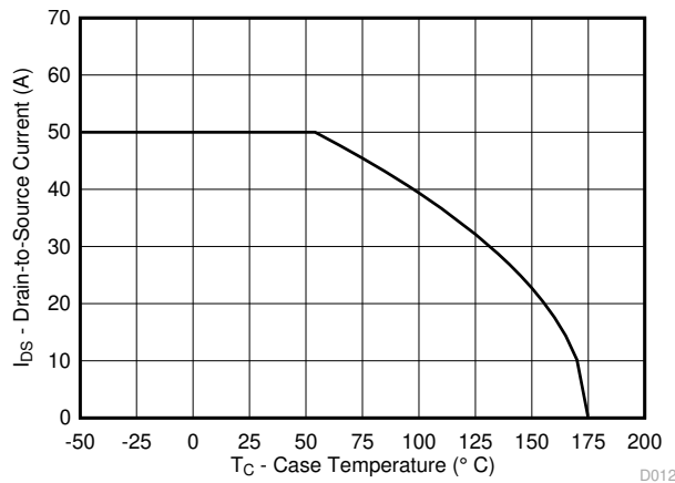
4-12. Maximum Drain Current vs Temperature
