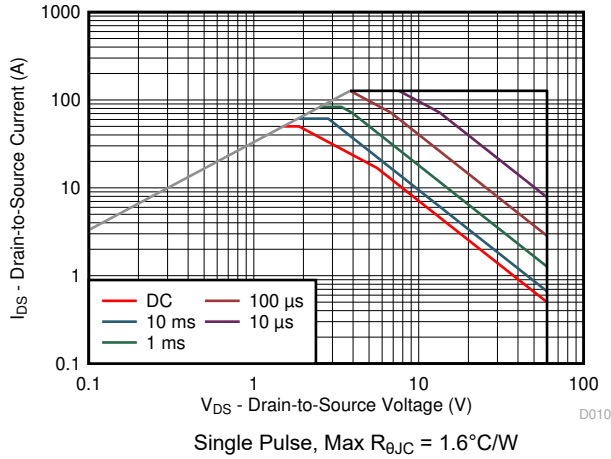
4-10. Maximum Safe Operating Area (SOA)
