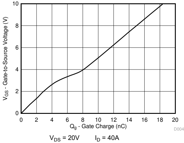
4-4. Gate Charge
