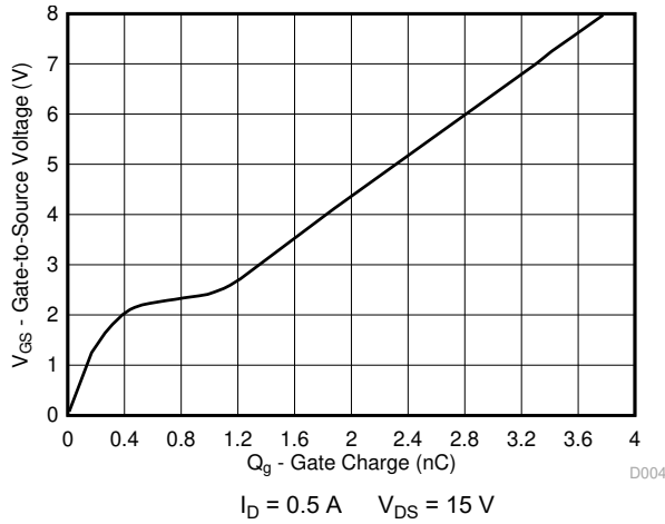
5-4. Gate Charge
