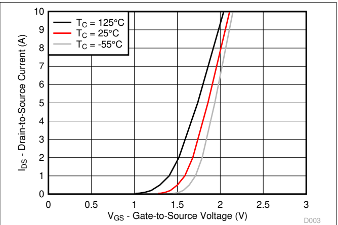
5-3. Transfer Characteristics
