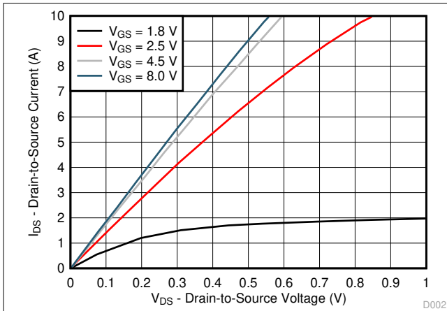
5-2. Saturation Characteristics
