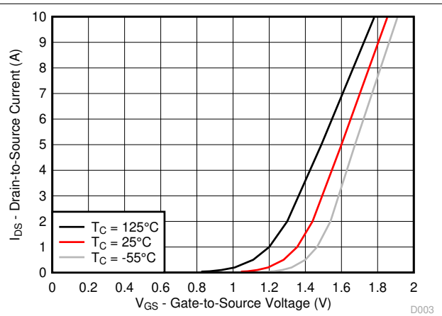
Figure 5-3. Transfer Characteristics
